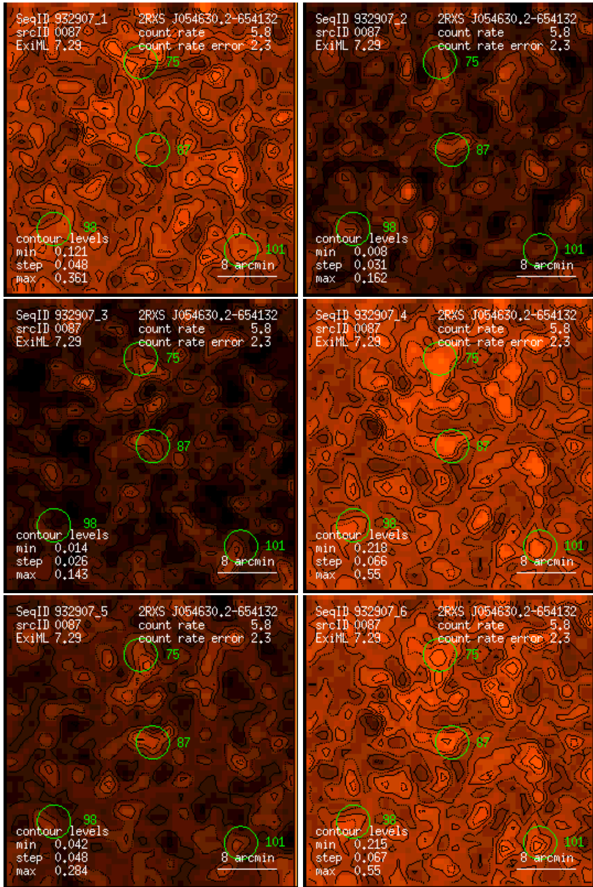
Figure 87: RASS 932907: detection 0087: band rate images, Gaussian filter: (1) PSPC channels 11 – 41, (2) 52 – 90, (3) 91 – 201, (4) 11 – 235, (5) 52 – 201, (6) 11 – 201. Broad band rates in counts/ks. Band rate contour levels in counts/ks/arcmin 2 .
