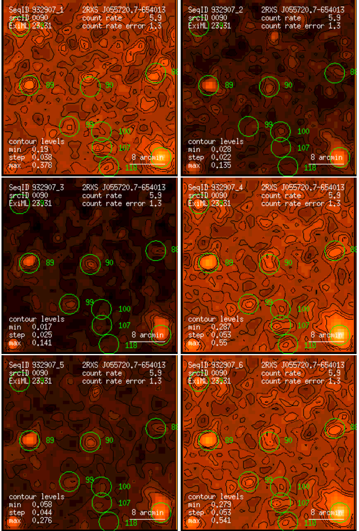
Figure 90: RASS 932907: detection 0090: band rate images, Gaussian filter: (1) PSPC channels 11 – 41, (2) 52 – 90, (3) 91 – 201, (4) 11 – 235, (5) 52 – 201, (6) 11 – 201. Broad band rates in counts/ks. Band rate contour levels in counts/ks/arcmin 2 .
