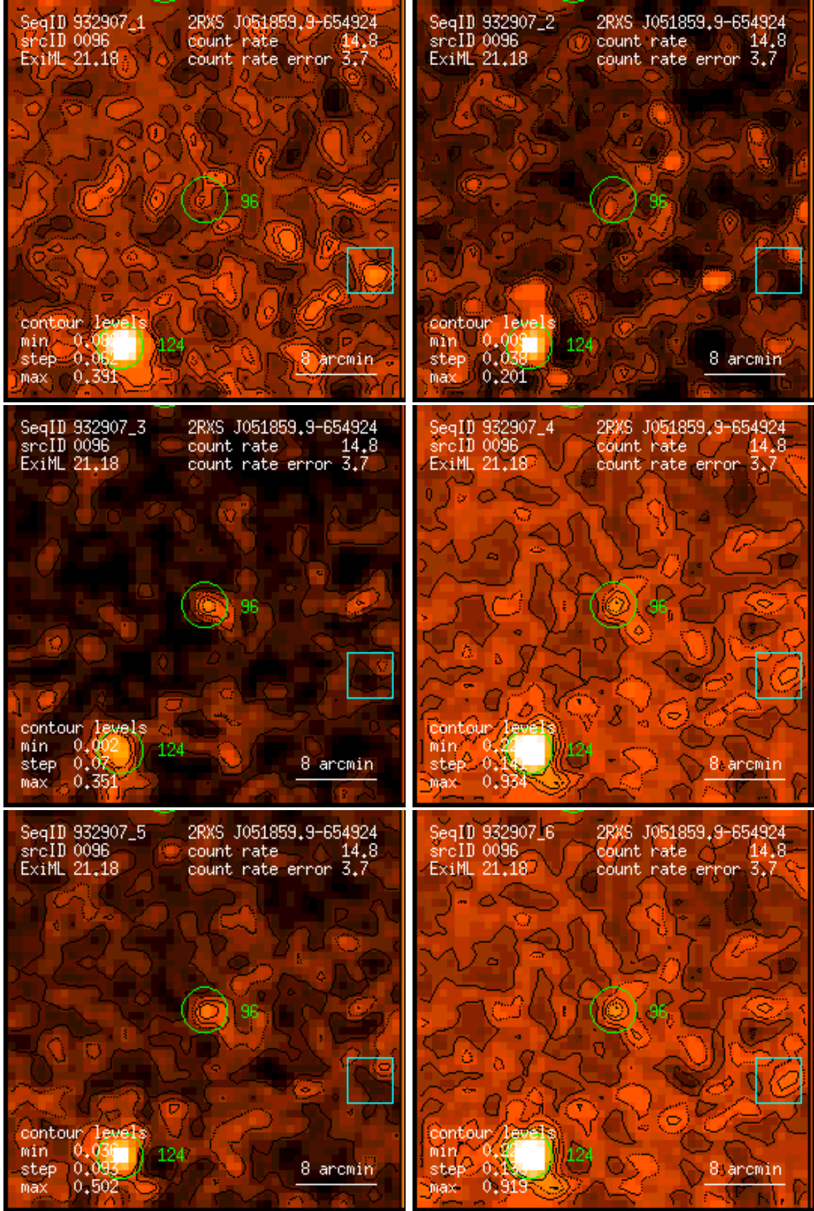
Figure 96: RASS 932907: detection 0096: band rate images, Gaussian filter: (1) PSPC channels 11 – 41, (2) 52 – 90, (3) 91 – 201, (4) 11 – 235, (5) 52 – 201, (6) 11 – 201. Broad band rates in counts/ks. Band rate contour levels in counts/ks/arcmin 2 .
