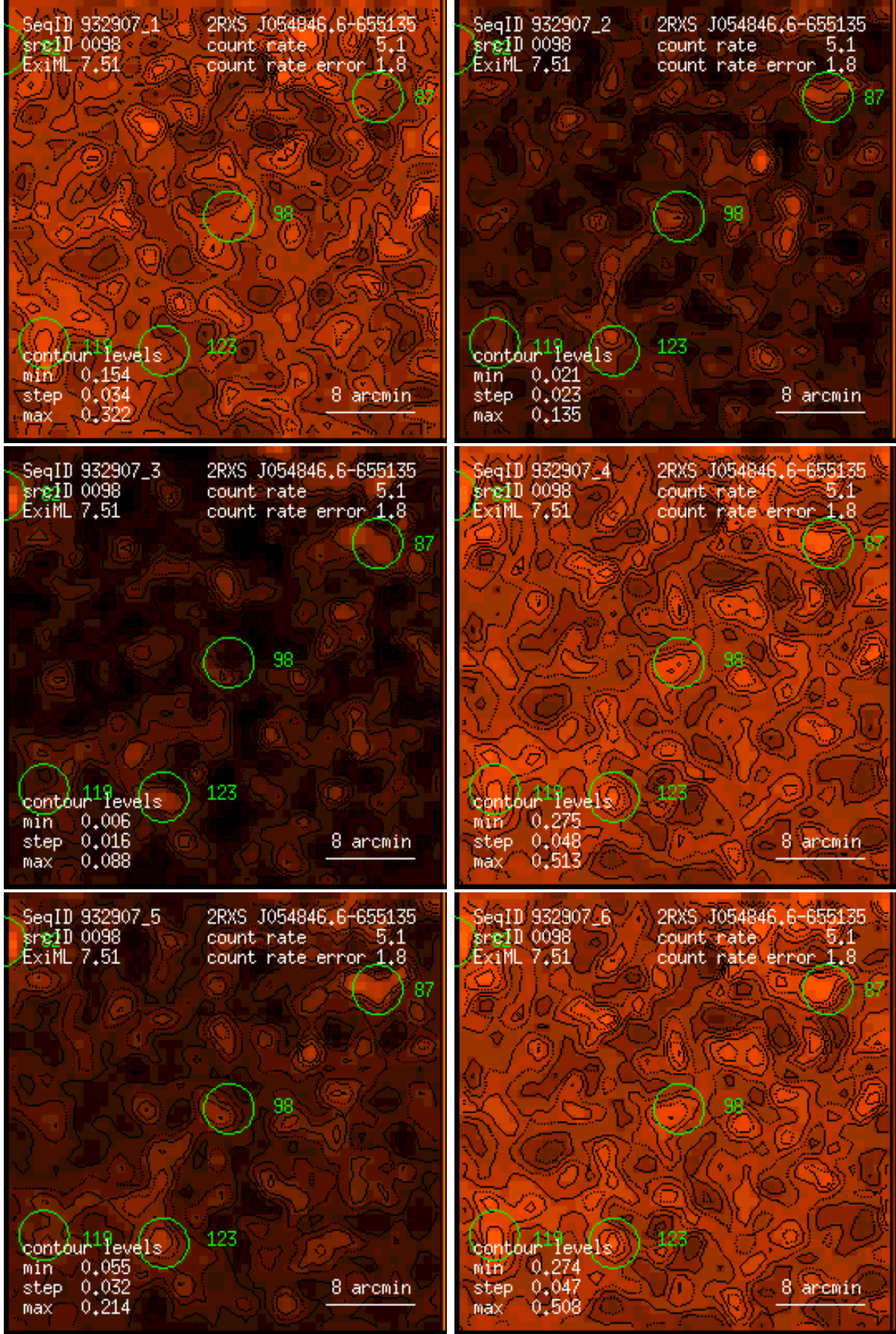
Figure 98: RASS 932907: detection 0098: band rate images, Gaussian filter: (1) PSPC channels 11 – 41, (2) 52 – 90, (3) 91 – 201, (4) 11 – 235, (5) 52 – 201, (6) 11 – 201. Broad band rates in counts/ks. Band rate contour levels in counts/ks/arcmin 2 .
