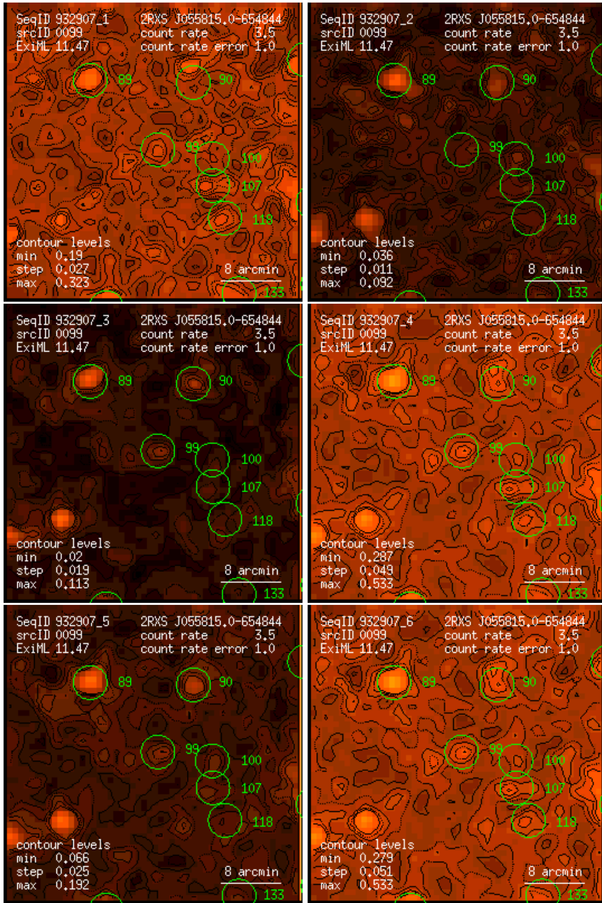
Figure 99: RASS 932907: detection 0099: band rate images, Gaussian filter: (1) PSPC channels 11 – 41, (2) 52 – 90, (3) 91 – 201, (4) 11 – 235, (5) 52 – 201, (6) 11 – 201. Broad band rates in counts/ks. Band rate contour levels in counts/ks/arcmin 2 .
