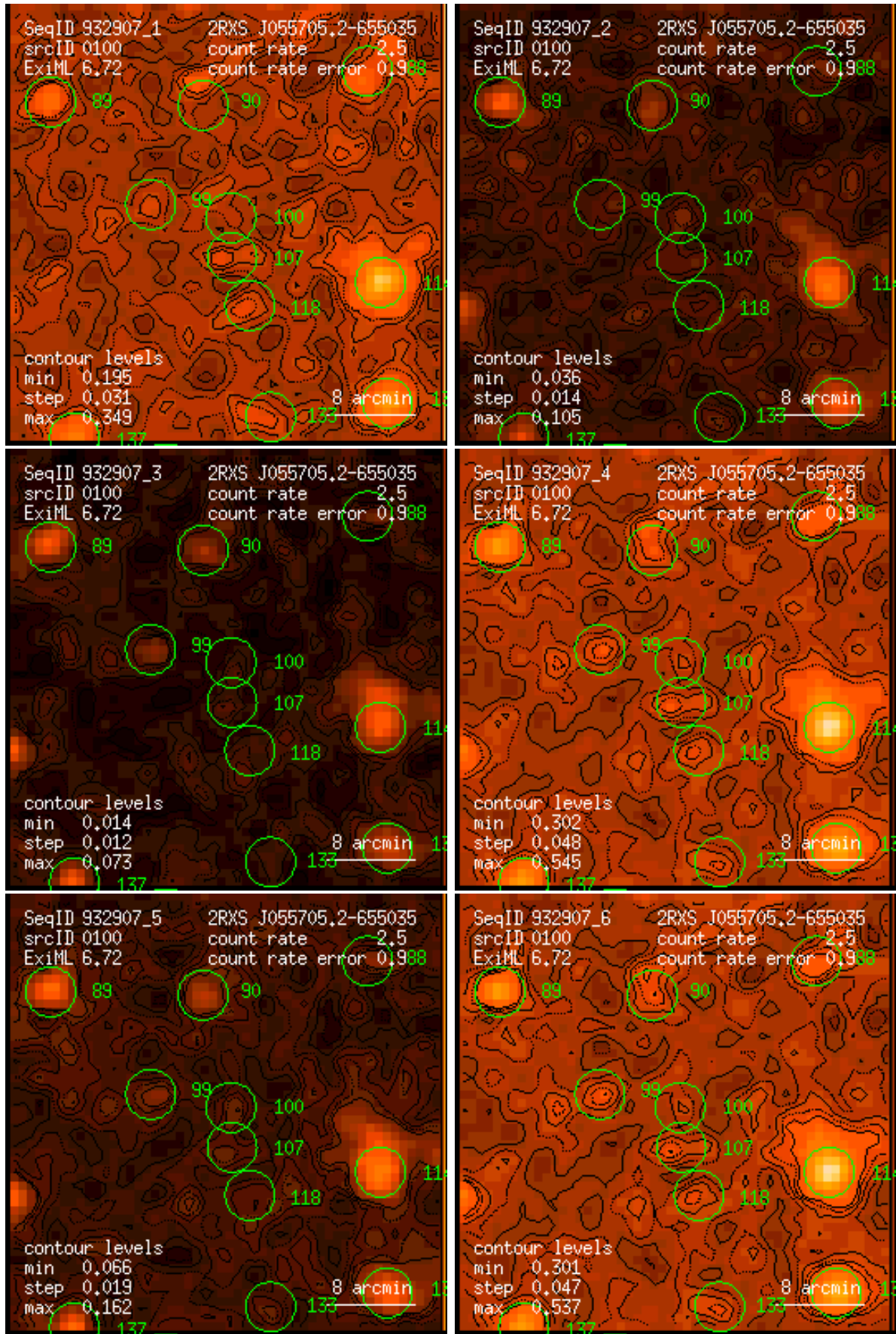
Figure 100: RASS 932907: detection 0100: band rate images, Gaussian filter: (1) PSPC channels 11 – 41, (2) 52 – 90, (3) 91 – 201, (4) 11 – 235, (5) 52 – 201, (6) 11 – 201. Broad band rates in counts/ks. Band rate contour levels in counts/ks/arcmin 2 .
