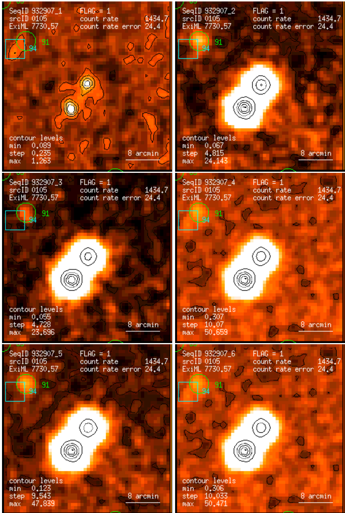
Figure 105: RASS 932907: detection 0105: band rate images, Gaussian filter: (1) PSPC channels 11 – 41, (2) 52 – 90, (3) 91 – 201, (4) 11 – 235, (5) 52 – 201, (6) 11 – 201. Broad band rates in counts/ks. Band rate contour levels in counts/ks/arcmin 2 .
