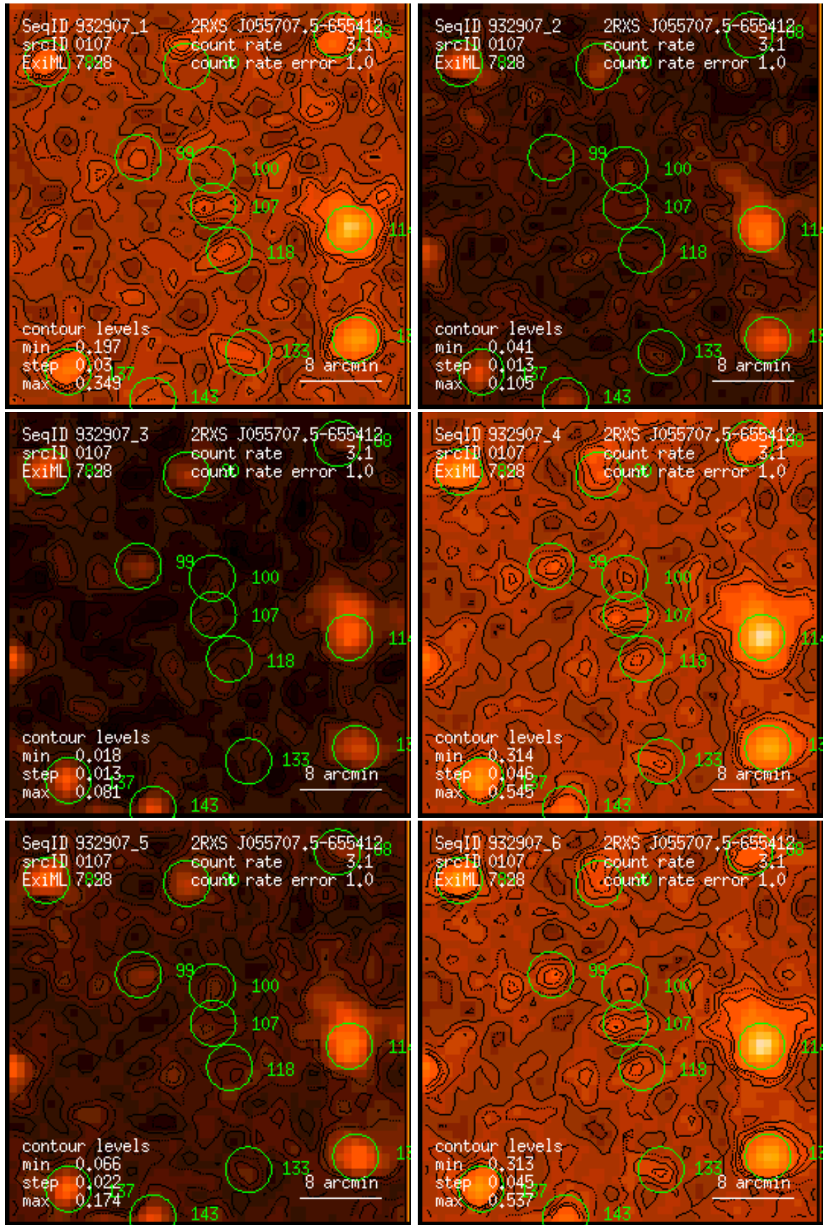
Figure 107: RASS 932907: detection 0107: band rate images, Gaussian filter: (1) PSPC channels 11 – 41, (2) 52 – 90, (3) 91 – 201, (4) 11 – 235, (5) 52 – 201, (6) 11 – 201. Broad band rates in counts/ks. Band rate contour levels in counts/ks/arcmin 2 .
