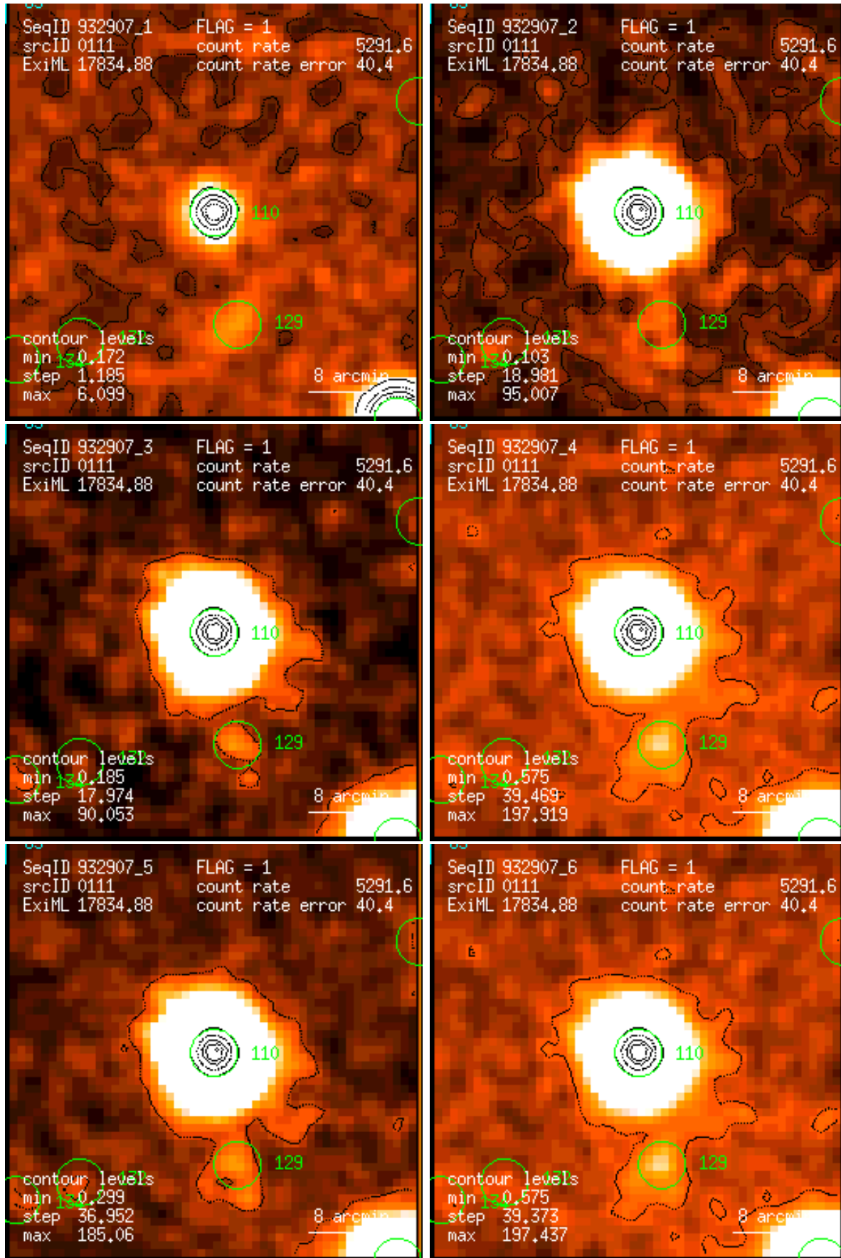
Figure 111: RASS 932907: detection 0111: band rate images, Gaussian filter: (1) PSPC channels 11 – 41, (2) 52 – 90, (3) 91 – 201, (4) 11 – 235, (5) 52 – 201, (6) 11 – 201. Broad band rates in counts/ks. Band rate contour levels in counts/ks/arcmin 2 .
