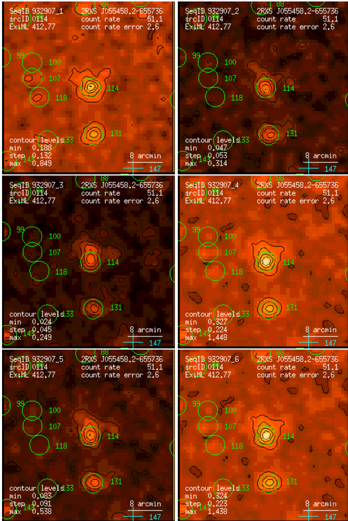
Figure 114: RASS 932907: detection 0114: band rate images, Gaussian filter: (1) PSPC channels 11 – 41, (2) 52 – 90, (3) 91 – 201, (4) 11 – 235, (5) 52 – 201, (6) 11 – 201. Broad band rates in counts/ks. Band rate contour levels in counts/ks/arcmin 2 .
