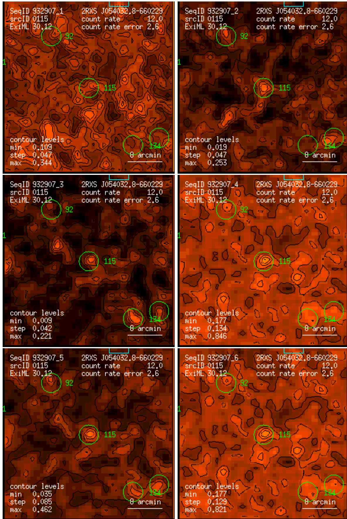
Figure 115: RASS 932907: detection 0115: band rate images, Gaussian filter: (1) PSPC channels 11 – 41, (2) 52 – 90, (3) 91 – 201, (4) 11 – 235, (5) 52 – 201, (6) 11 – 201. Broad band rates in counts/ks. Band rate contour levels in counts/ks/arcmin 2 .
