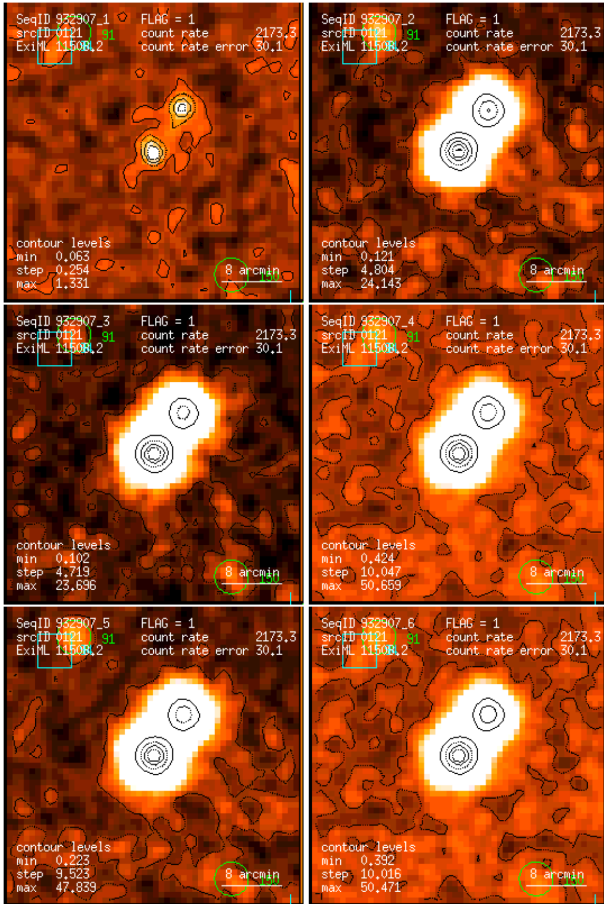
Figure 121: RASS 932907: detection 0121: band rate images, Gaussian filter: (1) PSPC channels 11 – 41, (2) 52 – 90, (3) 91 – 201, (4) 11 – 235, (5) 52 – 201, (6) 11 – 201. Broad band rates in counts/ks. Band rate contour levels in counts/ks/arcmin 2 .
