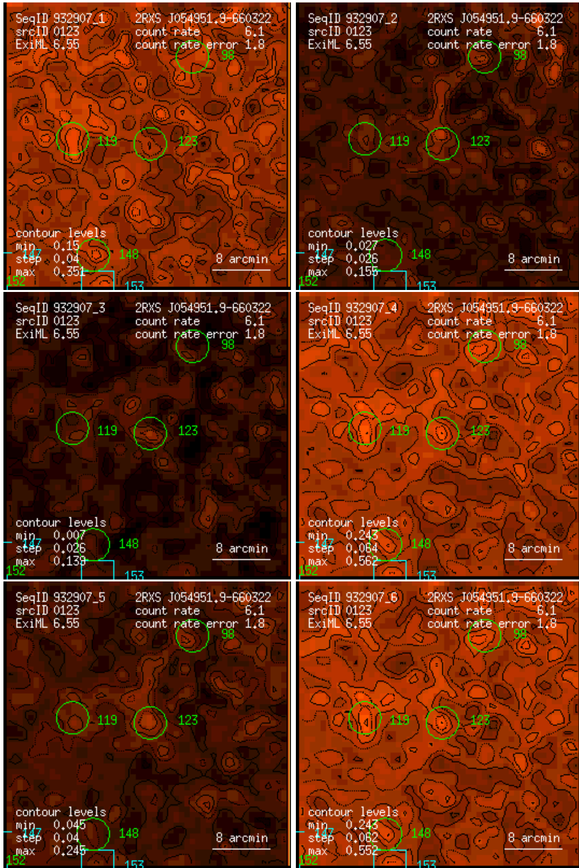
Figure 123: RASS 932907: detection 0123: band rate images, Gaussian filter: (1) PSPC channels 11 – 41, (2) 52 – 90, (3) 91 – 201, (4) 11 – 235, (5) 52 – 201, (6) 11 – 201. Broad band rates in counts/ks. Band rate contour levels in counts/ks/arcmin 2 .
