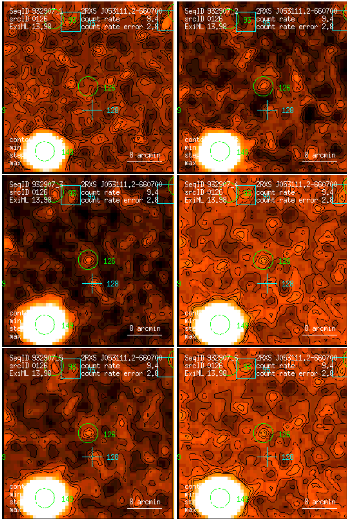
Figure 126: RASS 932907: detection 0126: band rate images, Gaussian filter: (1) PSPC channels 11 – 41, (2) 52 – 90, (3) 91 – 201, (4) 11 – 235, (5) 52 – 201, (6) 11 – 201. Broad band rates in counts/ks. Band rate contour levels in counts/ks/arcmin 2 .
