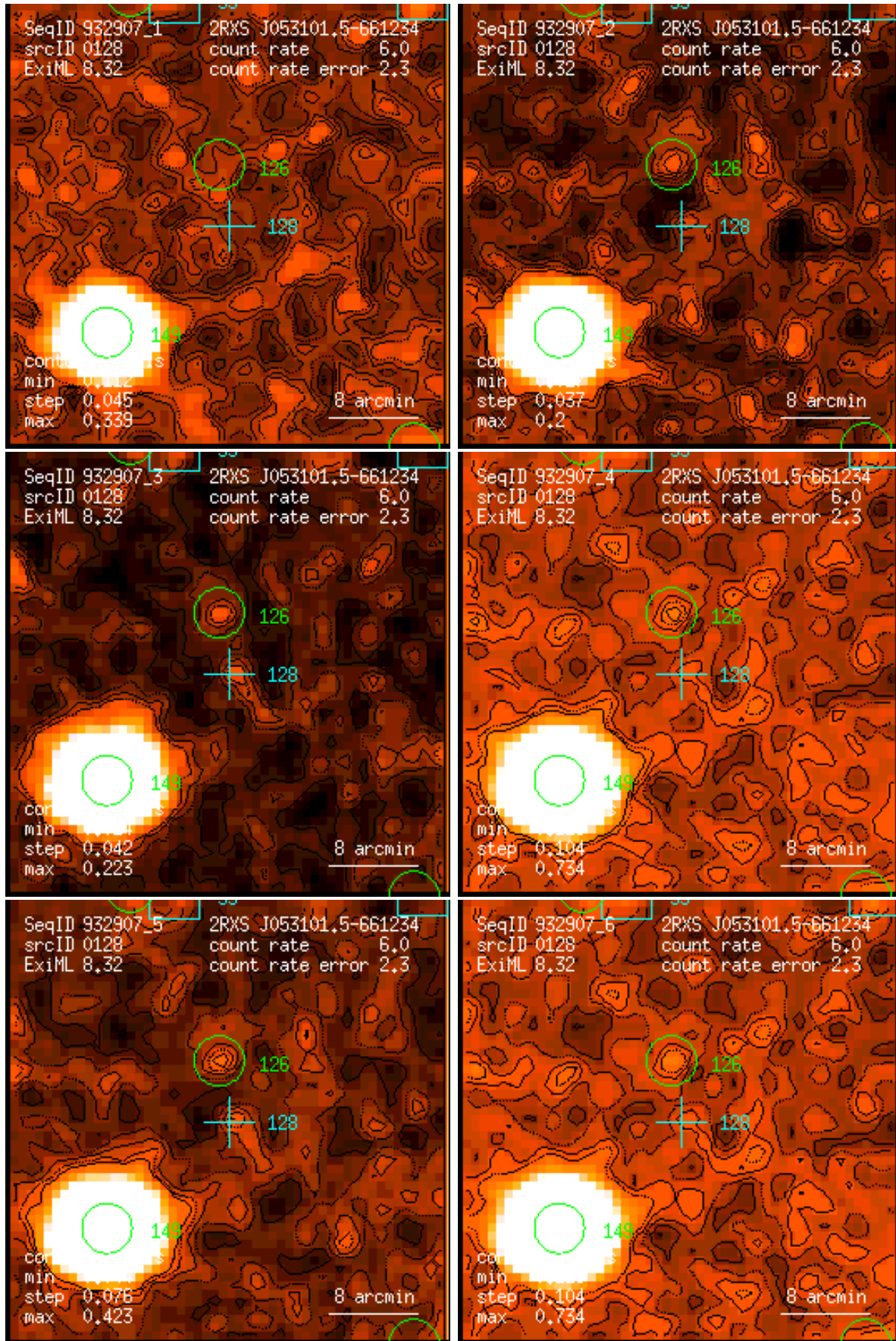
Figure 128: RASS 932907: detection 0128: band rate images, Gaussian filter: (1) PSPC channels 11 – 41, (2) 52 – 90, (3) 91 – 201, (4) 11 – 235, (5) 52 – 201, (6) 11 – 201. Broad band rates in counts/ks. Band rate contour levels in counts/ks/arcmin 2 .
