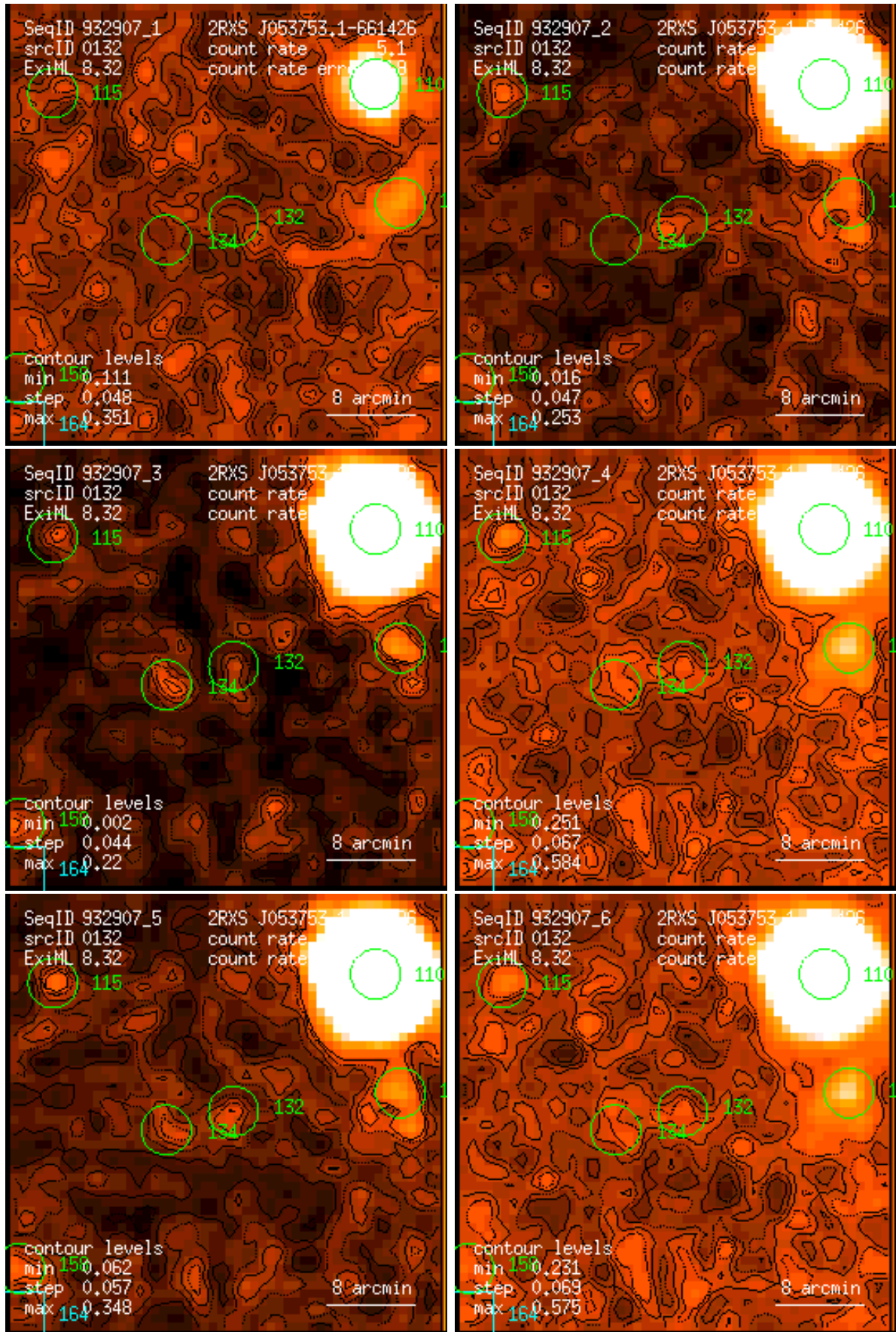
Figure 132: RASS 932907: detection 0132: band rate images, Gaussian filter: (1) PSPC channels 11 – 41, (2) 52 – 90, (3) 91 – 201, (4) 11 – 235, (5) 52 – 201, (6) 11 – 201. Broad band rates in counts/ks. Band rate contour levels in counts/ks/arcmin 2 .
