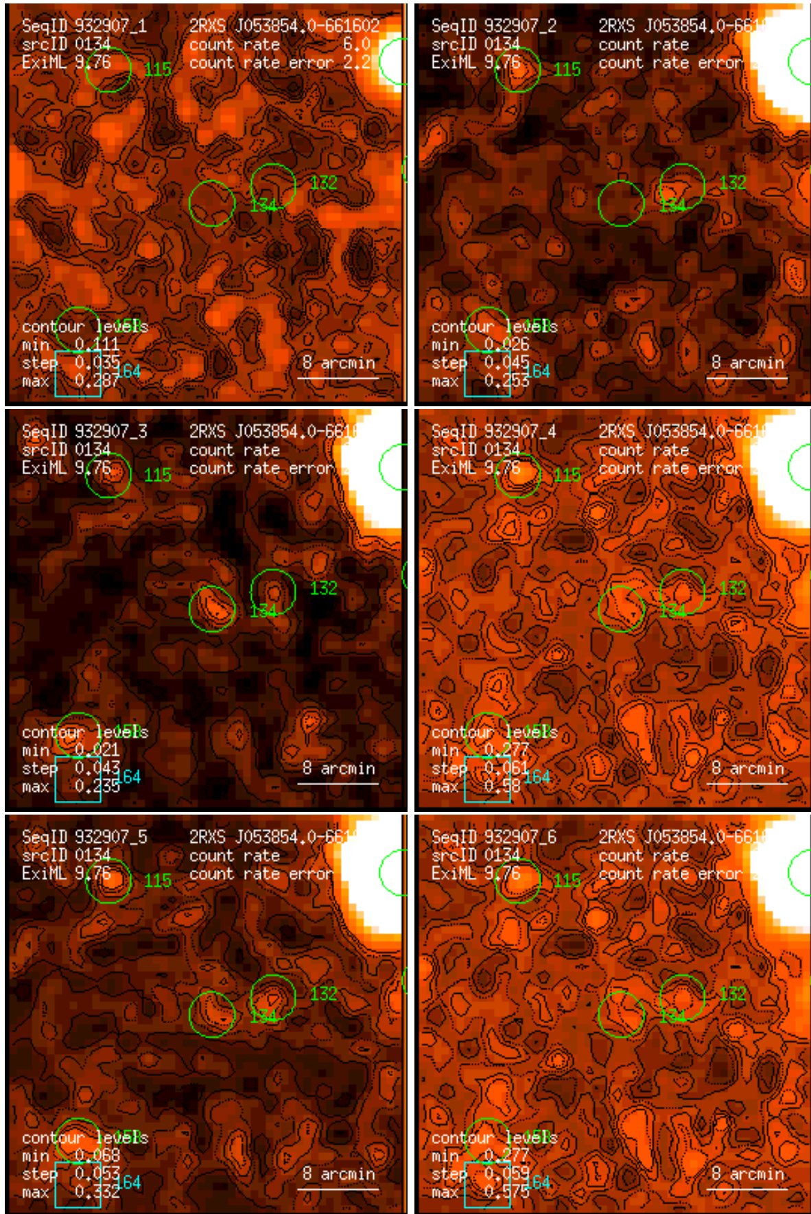
Figure 134: RASS 932907: detection 0134: band rate images, Gaussian filter: (1) PSPC channels 11 – 41, (2) 52 – 90, (3) 91 – 201, (4) 11 – 235, (5) 52 – 201, (6) 11 – 201. Broad band rates in counts/ks. Band rate contour levels in counts/ks/arcmin 2 .
