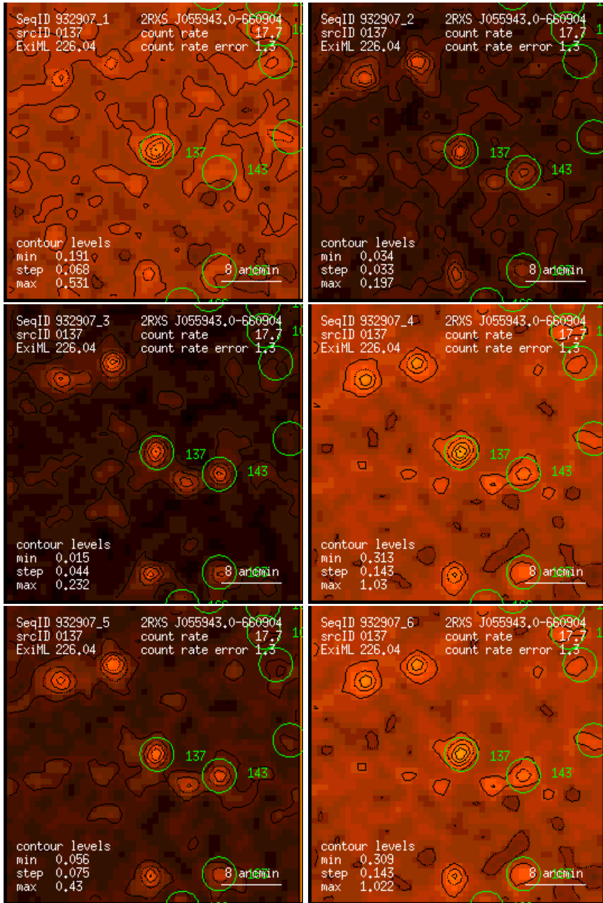
Figure 137: RASS 932907: detection 0137: band rate images, Gaussian filter: (1) PSPC channels 11 – 41, (2) 52 – 90, (3) 91 – 201, (4) 11 – 235, (5) 52 – 201, (6) 11 – 201. Broad band rates in counts/ks. Band rate contour levels in counts/ks/arcmin 2 .
