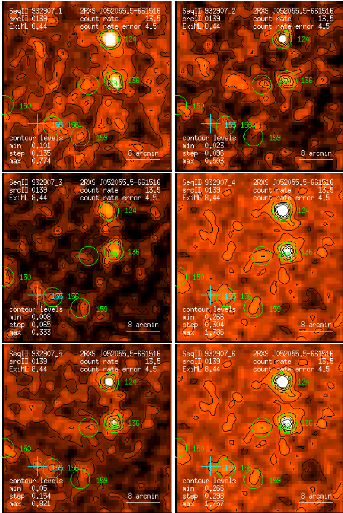
Figure 139: RASS 932907: detection 0139: band rate images, Gaussian filter: (1) PSPC channels 11 – 41, (2) 52 – 90, (3) 91 – 201, (4) 11 – 235, (5) 52 – 201, (6) 11 – 201. Broad band rates in counts/ks. Band rate contour levels in counts/ks/arcmin 2 .
