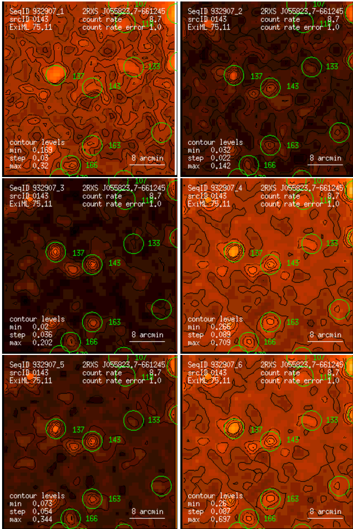
Figure 143: RASS 932907: detection 0143: band rate images, Gaussian filter: (1) PSPC channels 11 – 41, (2) 52 – 90, (3) 91 – 201, (4) 11 – 235, (5) 52 – 201, (6) 11 – 201. Broad band rates in counts/ks. Band rate contour levels in counts/ks/arcmin 2 .
