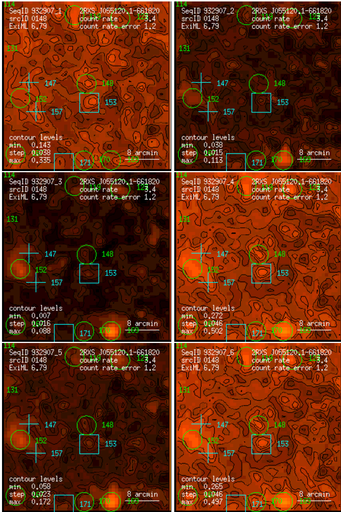
Figure 148: RASS 932907: detection 0148: band rate images, Gaussian filter: (1) PSPC channels 11 – 41, (2) 52 – 90, (3) 91 – 201, (4) 11 – 235, (5) 52 – 201, (6) 11 – 201. Broad band rates in counts/ks. Band rate contour levels in counts/ks/arcmin 2 .
