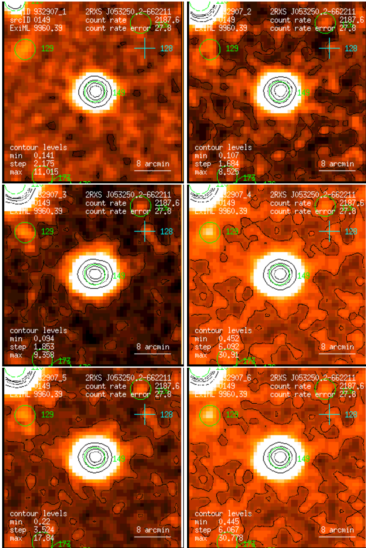
Figure 149: RASS 932907: detection 0149: band rate images, Gaussian filter: (1) PSPC channels 11 – 41, (2) 52 – 90, (3) 91 – 201, (4) 11 – 235, (5) 52 – 201, (6) 11 – 201. Broad band rates in counts/ks. Band rate contour levels in counts/ks/arcmin 2 .
