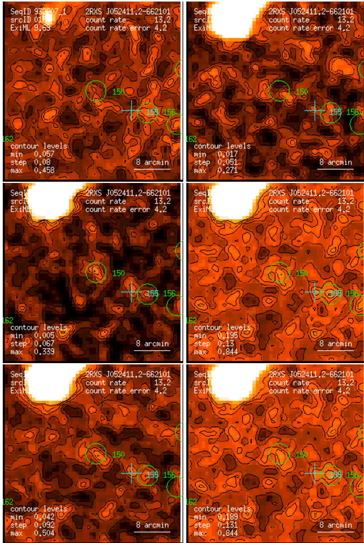
Figure 150: RASS 932907: detection 0150: band rate images, Gaussian filter: (1) PSPC channels 11 – 41, (2) 52 – 90, (3) 91 – 201, (4) 11 – 235, (5) 52 – 201, (6) 11 – 201. Broad band rates in counts/ks. Band rate contour levels in counts/ks/arcmin 2 .
