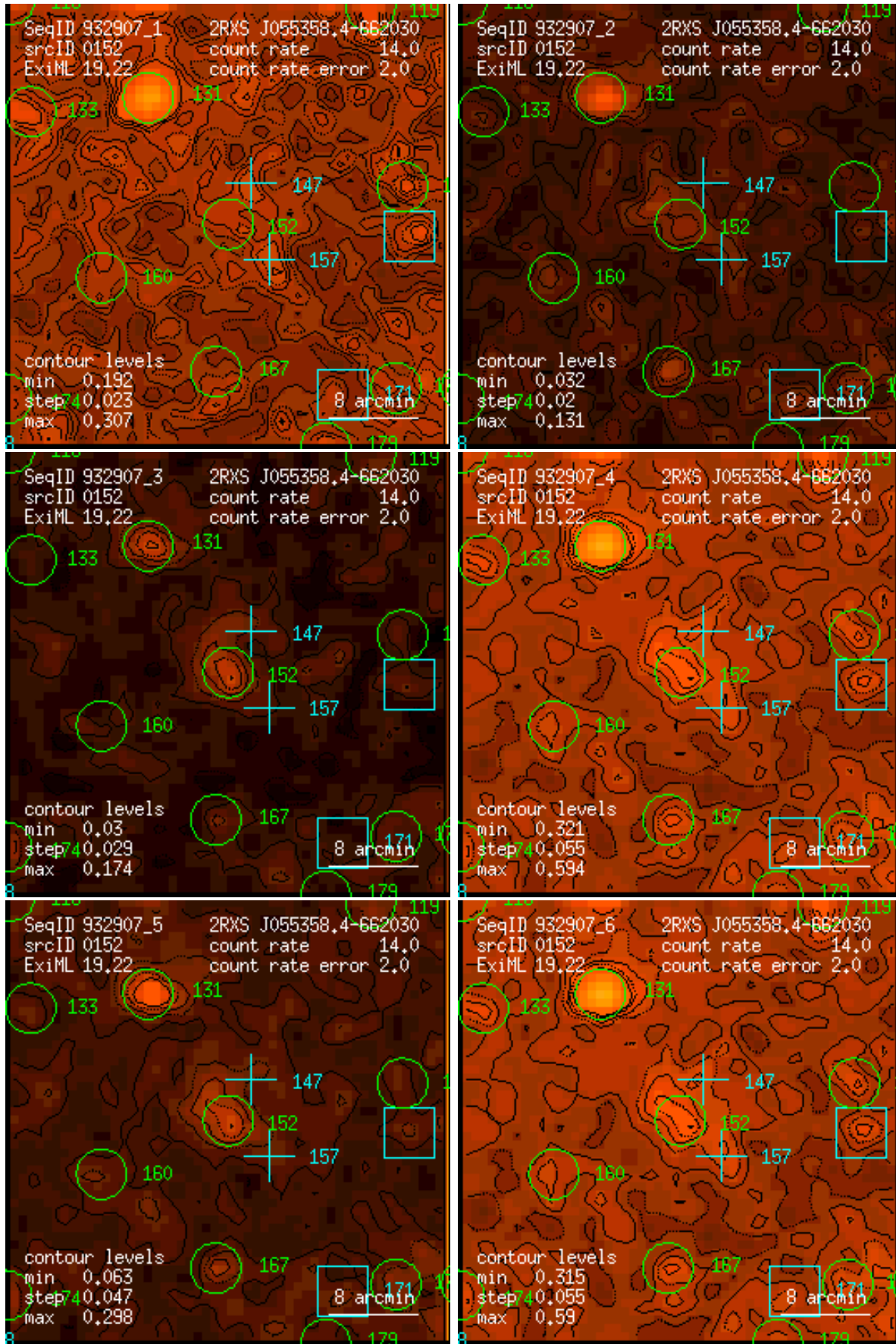
Figure 152: RASS 932907: detection 0152: band rate images, Gaussian filter: (1) PSPC channels 11 – 41, (2) 52 – 90, (3) 91 – 201, (4) 11 – 235, (5) 52 – 201, (6) 11 – 201. Broad band rates in counts/ks. Band rate contour levels in counts/ks/arcmin 2 .
