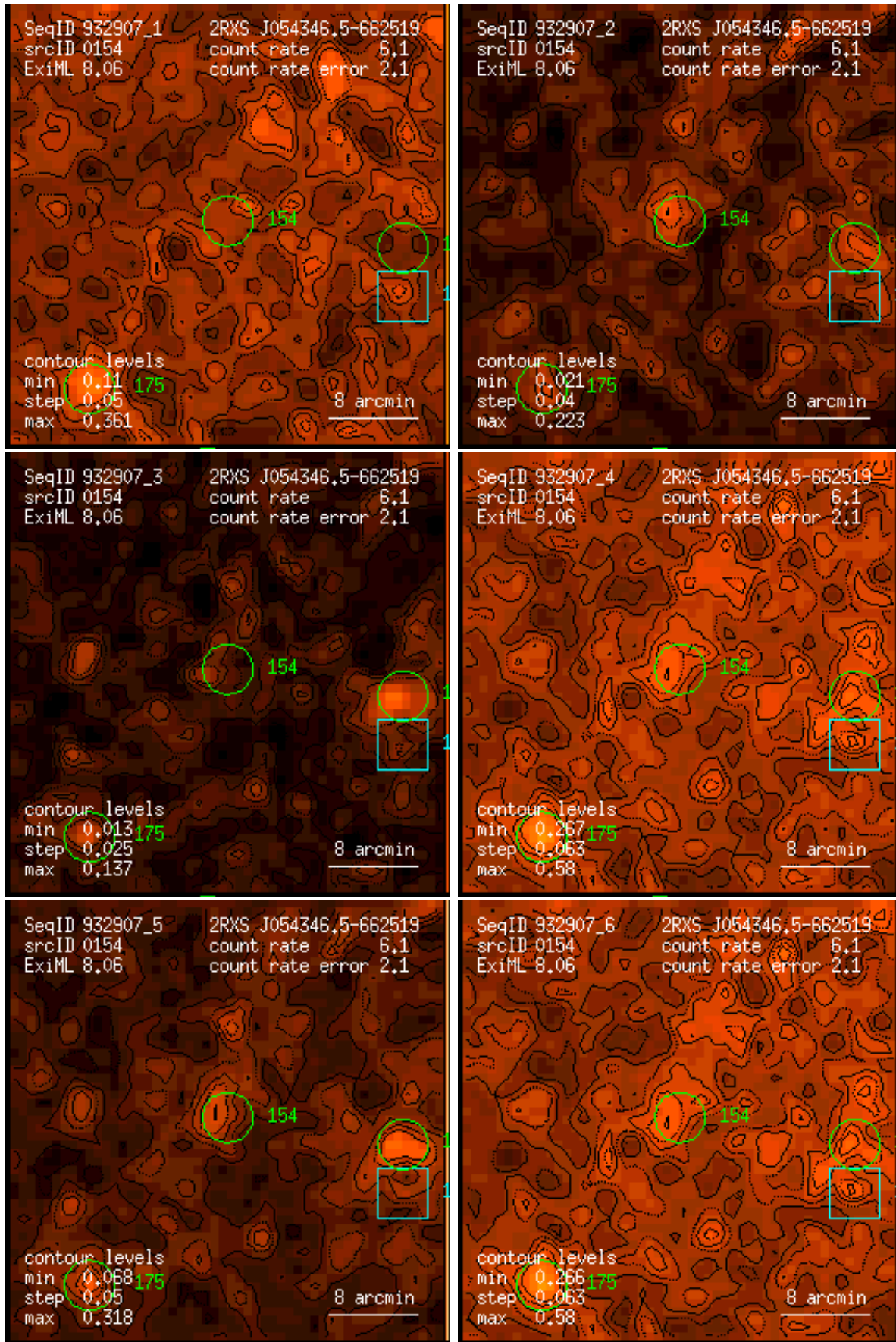
Figure 154: RASS 932907: detection 0154: band rate images, Gaussian filter: (1) PSPC channels 11 – 41, (2) 52 – 90, (3) 91 – 201, (4) 11 – 235, (5) 52 – 201, (6) 11 – 201. Broad band rates in counts/ks. Band rate contour levels in counts/ks/arcmin 2 .
