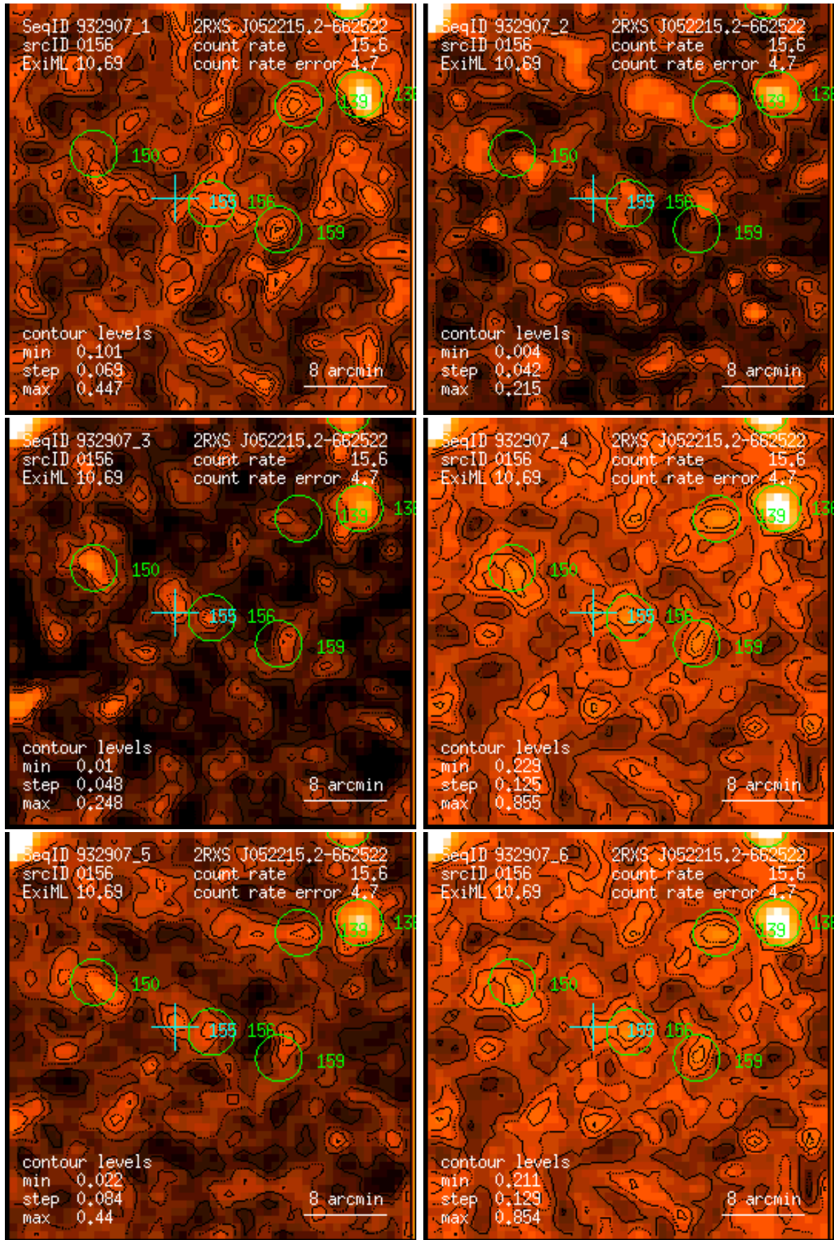
Figure 156: RASS 932907: detection 0156: band rate images, Gaussian filter: (1) PSPC channels 11 – 41, (2) 52 – 90, (3) 91 – 201, (4) 11 – 235, (5) 52 – 201, (6) 11 – 201. Broad band rates in counts/ks. Band rate contour levels in counts/ks/arcmin 2 .
