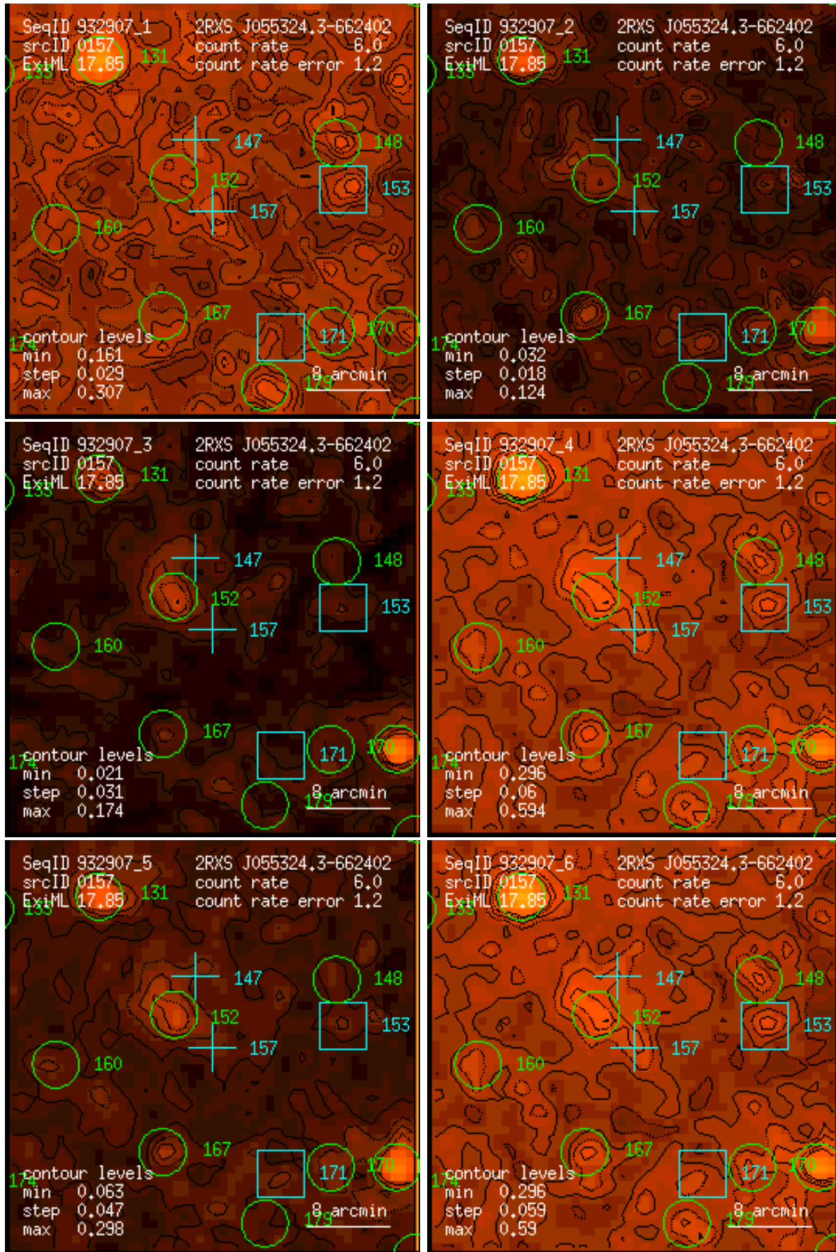
Figure 157: RASS 932907: detection 0157: band rate images, Gaussian filter: (1) PSPC channels 11 – 41, (2) 52 – 90, (3) 91 – 201, (4) 11 – 235, (5) 52 – 201, (6) 11 – 201. Broad band rates in counts/ks. Band rate contour levels in counts/ks/arcmin 2 .
