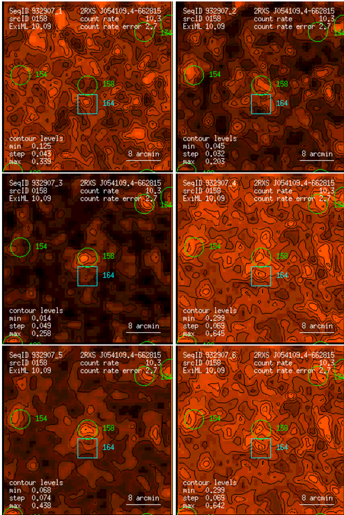
Figure 158: RASS 932907: detection 0158: band rate images, Gaussian filter: (1) PSPC channels 11 – 41, (2) 52 – 90, (3) 91 – 201, (4) 11 – 235, (5) 52 – 201, (6) 11 – 201. Broad band rates in counts/ks. Band rate contour levels in counts/ks/arcmin 2 .
