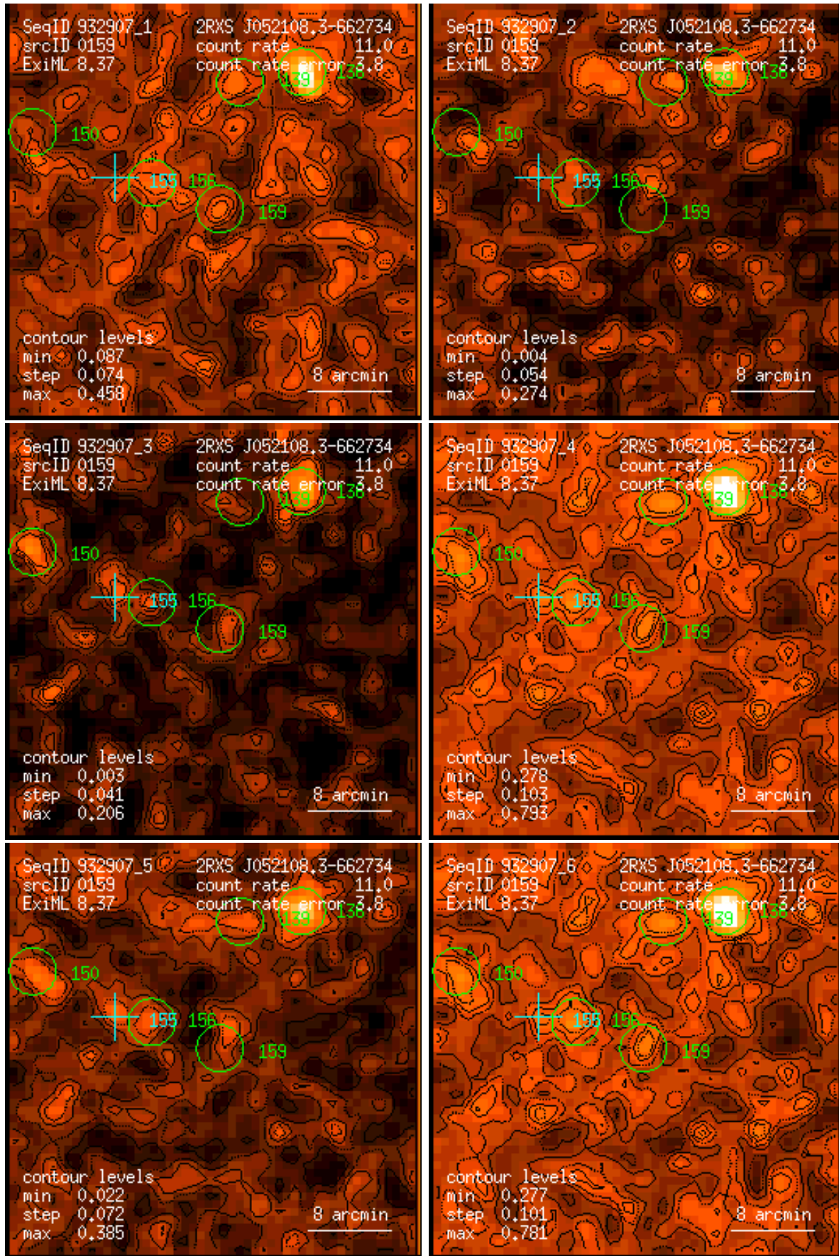
Figure 159: RASS 932907: detection 0159: band rate images, Gaussian filter: (1) PSPC channels 11 – 41, (2) 52 – 90, (3) 91 – 201, (4) 11 – 235, (5) 52 – 201, (6) 11 – 201. Broad band rates in counts/ks. Band rate contour levels in counts/ks/arcmin 2 .
