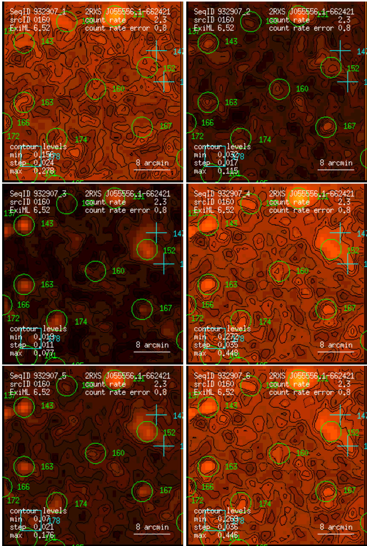
Figure 160: RASS 932907: detection 0160: band rate images, Gaussian filter: (1) PSPC channels 11 – 41, (2) 52 – 90, (3) 91 – 201, (4) 11 – 235, (5) 52 – 201, (6) 11 – 201. Broad band rates in counts/ks. Band rate contour levels in counts/ks/arcmin 2 .
