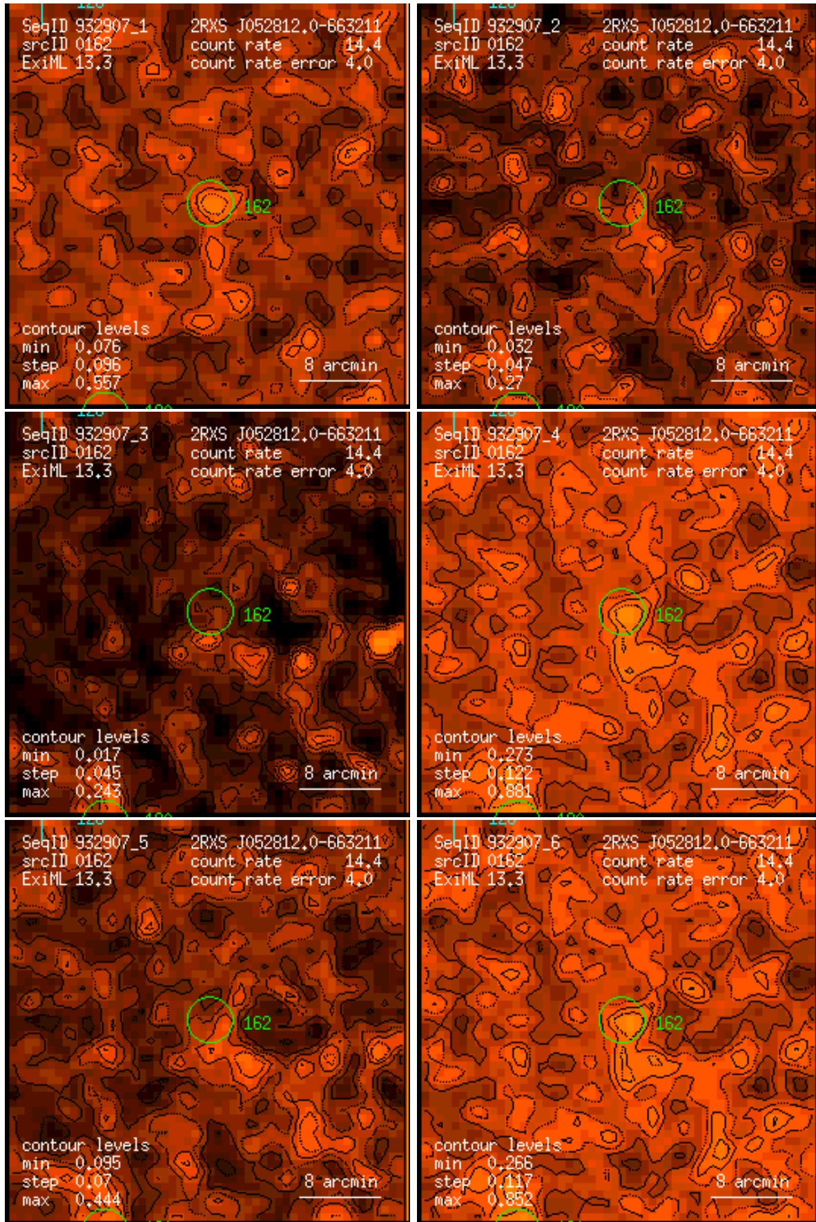
Figure 162: RASS 932907: detection 0162: band rate images, Gaussian filter: (1) PSPC channels 11 – 41, (2) 52 – 90, (3) 91 – 201, (4) 11 – 235, (5) 52 – 201, (6) 11 – 201. Broad band rates in counts/ks. Band rate contour levels in counts/ks/arcmin 2 .
