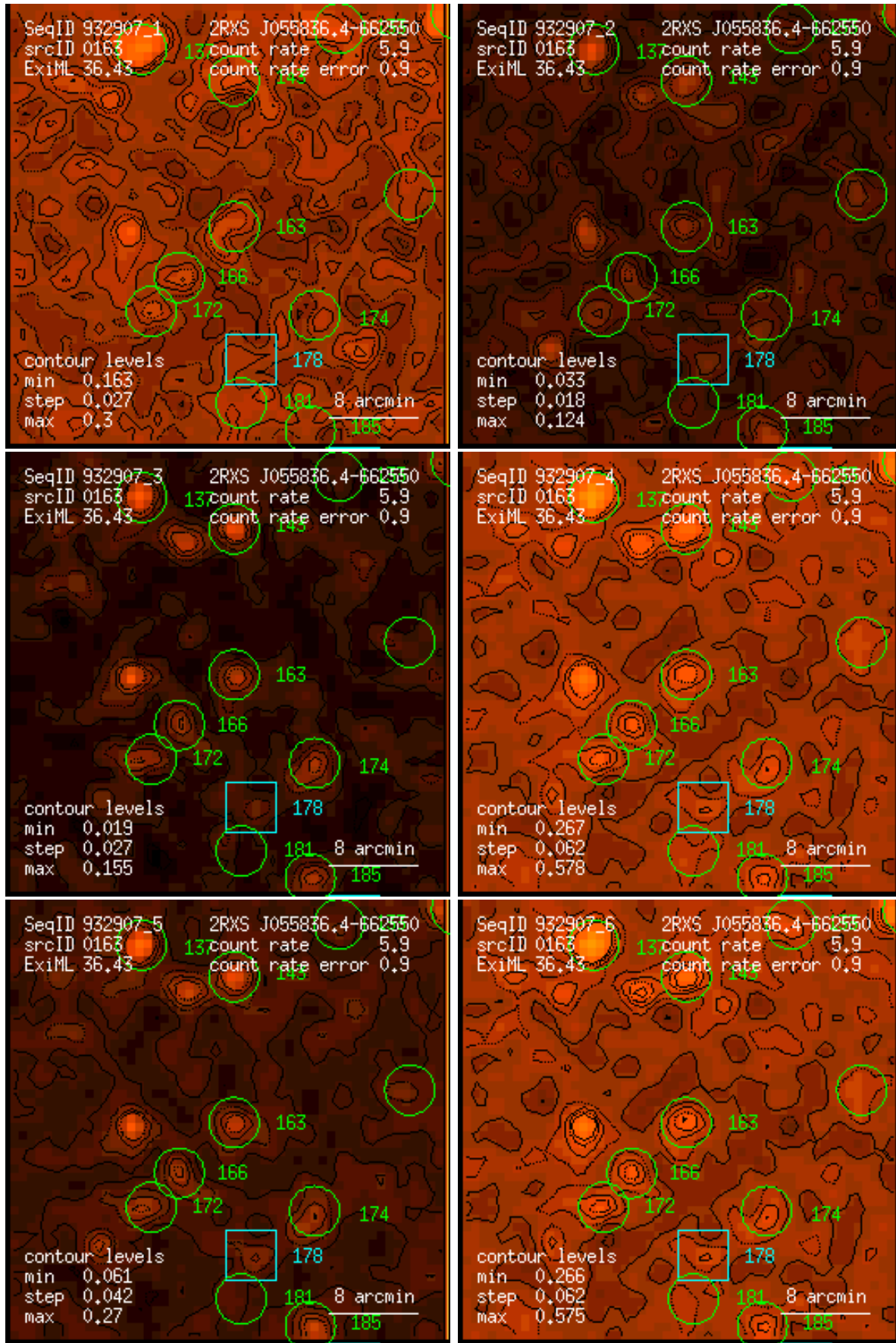
Figure 163: RASS 932907: detection 0163: band rate images, Gaussian filter: (1) PSPC channels 11 – 41, (2) 52 – 90, (3) 91 – 201, (4) 11 – 235, (5) 52 – 201, (6) 11 – 201. Broad band rates in counts/ks. Band rate contour levels in counts/ks/arcmin 2 .
