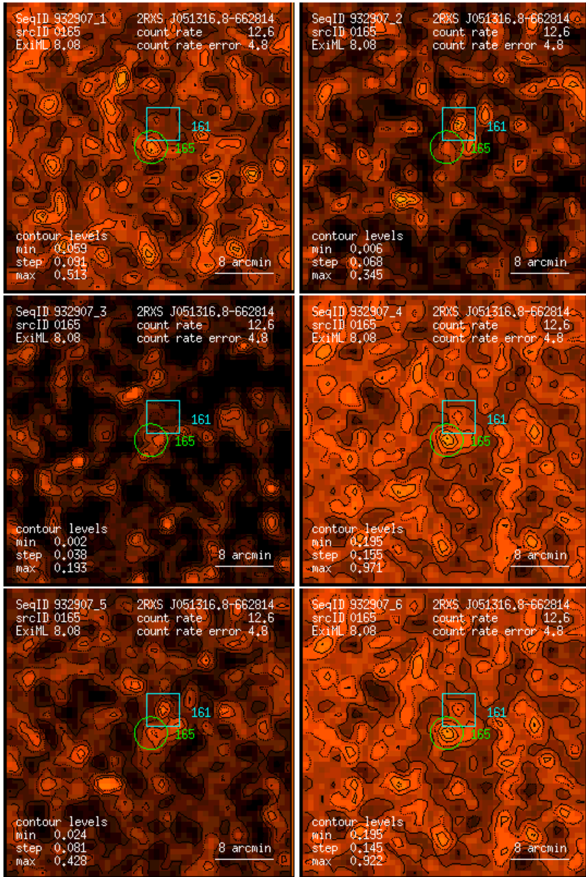
Figure 165: RASS 932907: detection 0165: band rate images, Gaussian filter: (1) PSPC channels 11 – 41, (2) 52 – 90, (3) 91 – 201, (4) 11 – 235, (5) 52 – 201, (6) 11 – 201. Broad band rates in counts/ks. Band rate contour levels in counts/ks/arcmin 2 .
