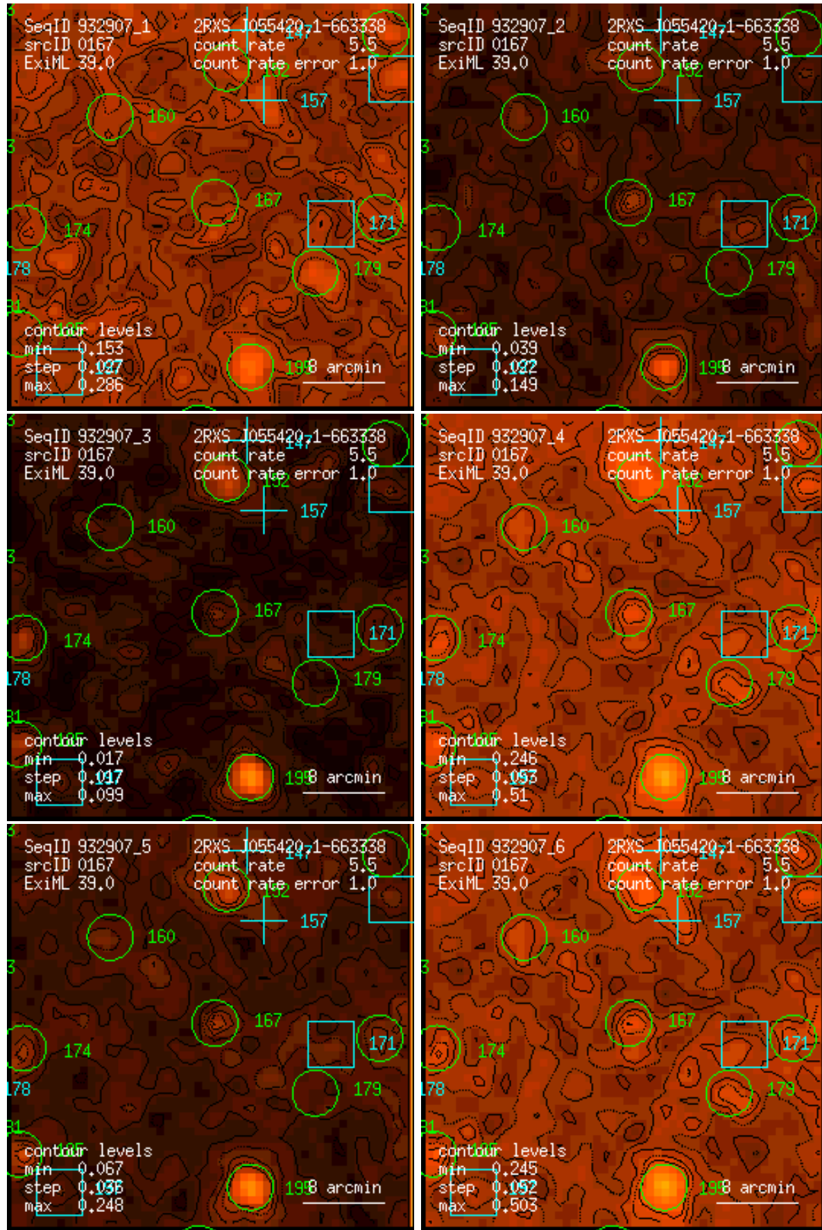
Figure 167: RASS 932907: detection 0167: band rate images, Gaussian filter: (1) PSPC channels 11 – 41, (2) 52 – 90, (3) 91 – 201, (4) 11 – 235, (5) 52 – 201, (6) 11 – 201. Broad band rates in counts/ks. Band rate contour levels in counts/ks/arcmin 2 .
