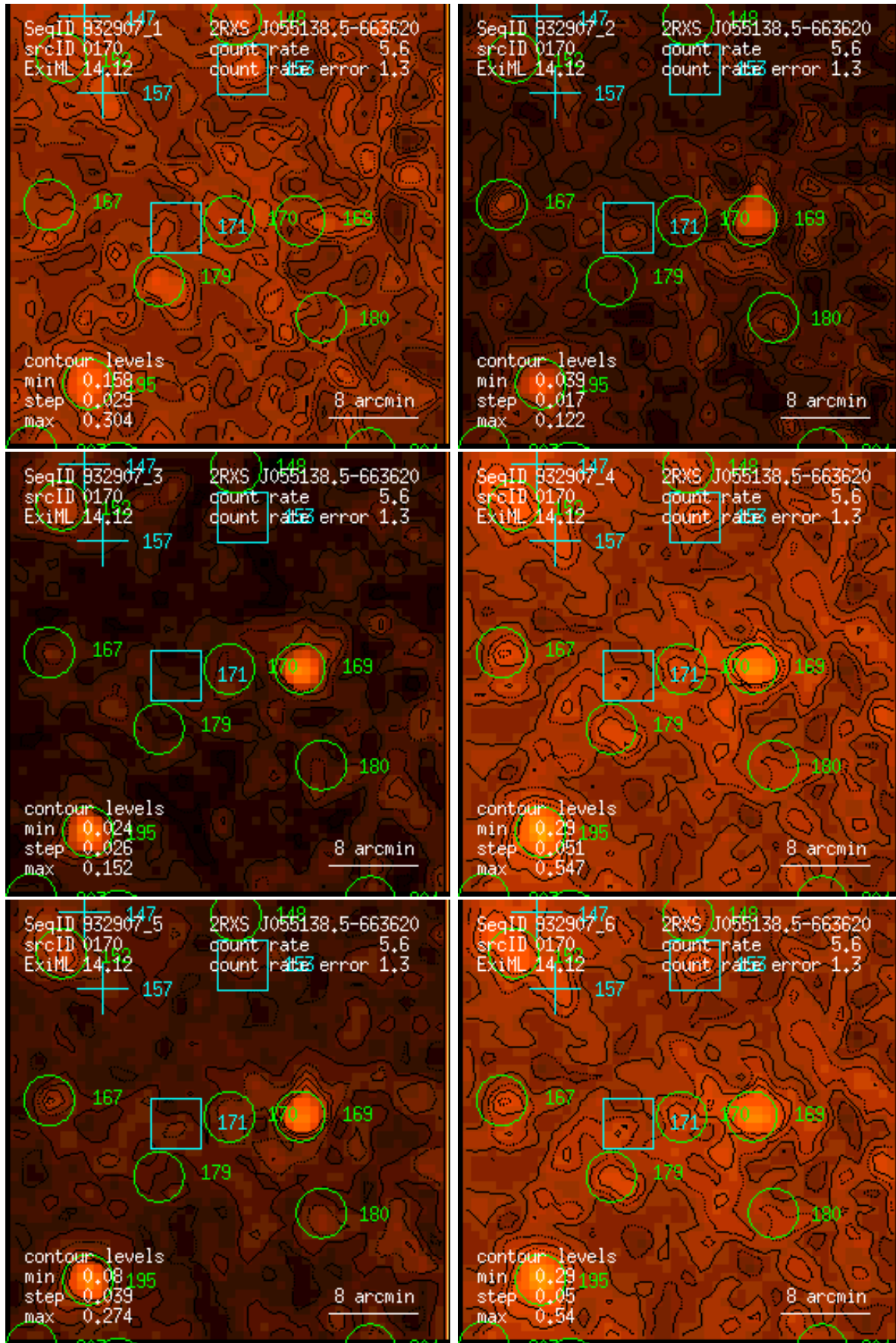
Figure 170: RASS 932907: detection 0170: band rate images, Gaussian filter: (1) PSPC channels 11 – 41, (2) 52 – 90, (3) 91 – 201, (4) 11 – 235, (5) 52 – 201, (6) 11 – 201. Broad band rates in counts/ks. Band rate contour levels in counts/ks/arcmin 2 .
