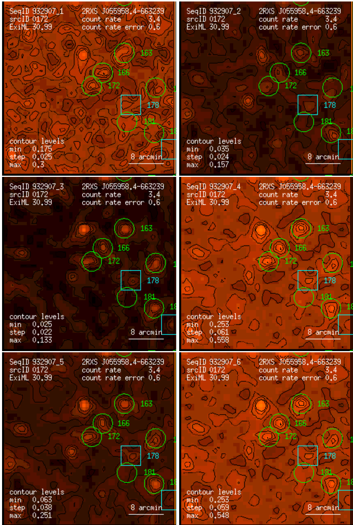
Figure 172: RASS 932907: detection 0172: band rate images, Gaussian filter: (1) PSPC channels 11 – 41, (2) 52 – 90, (3) 91 – 201, (4) 11 – 235, (5) 52 – 201, (6) 11 – 201. Broad band rates in counts/ks. Band rate contour levels in counts/ks/arcmin 2 .
