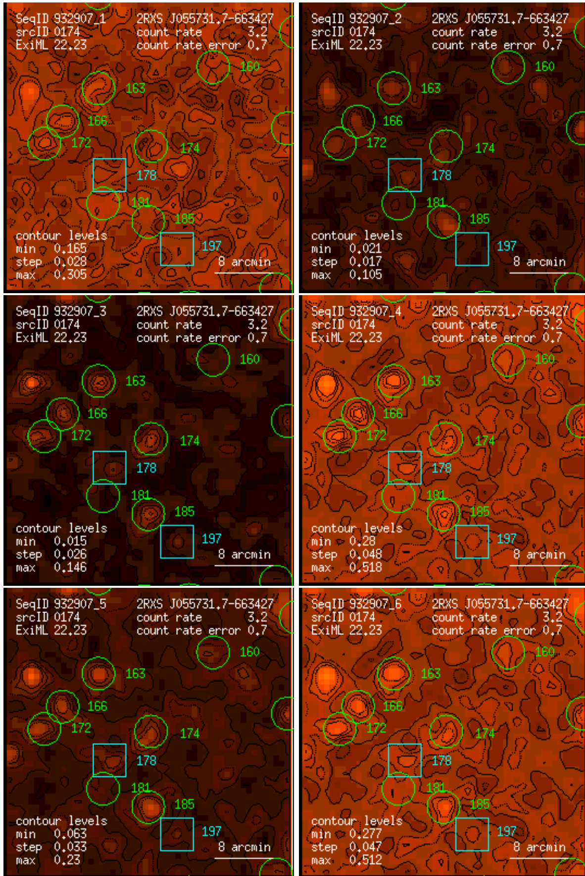
Figure 174: RASS 932907: detection 0174: band rate images, Gaussian filter: (1) PSPC channels 11 – 41, (2) 52 – 90, (3) 91 – 201, (4) 11 – 235, (5) 52 – 201, (6) 11 – 201. Broad band rates in counts/ks. Band rate contour levels in counts/ks/arcmin 2 .
