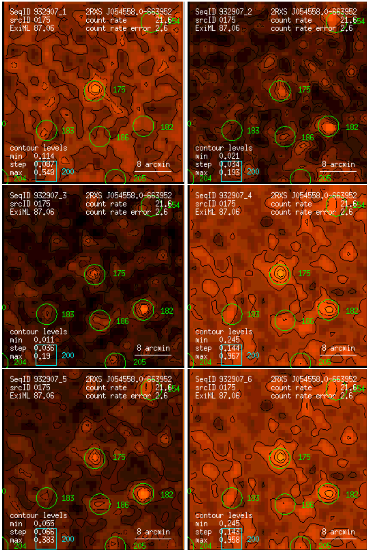
Figure 175: RASS 932907: detection 0175: band rate images, Gaussian filter: (1) PSPC channels 11 – 41, (2) 52 – 90, (3) 91 – 201, (4) 11 – 235, (5) 52 – 201, (6) 11 – 201. Broad band rates in counts/ks. Band rate contour levels in counts/ks/arcmin 2 .
