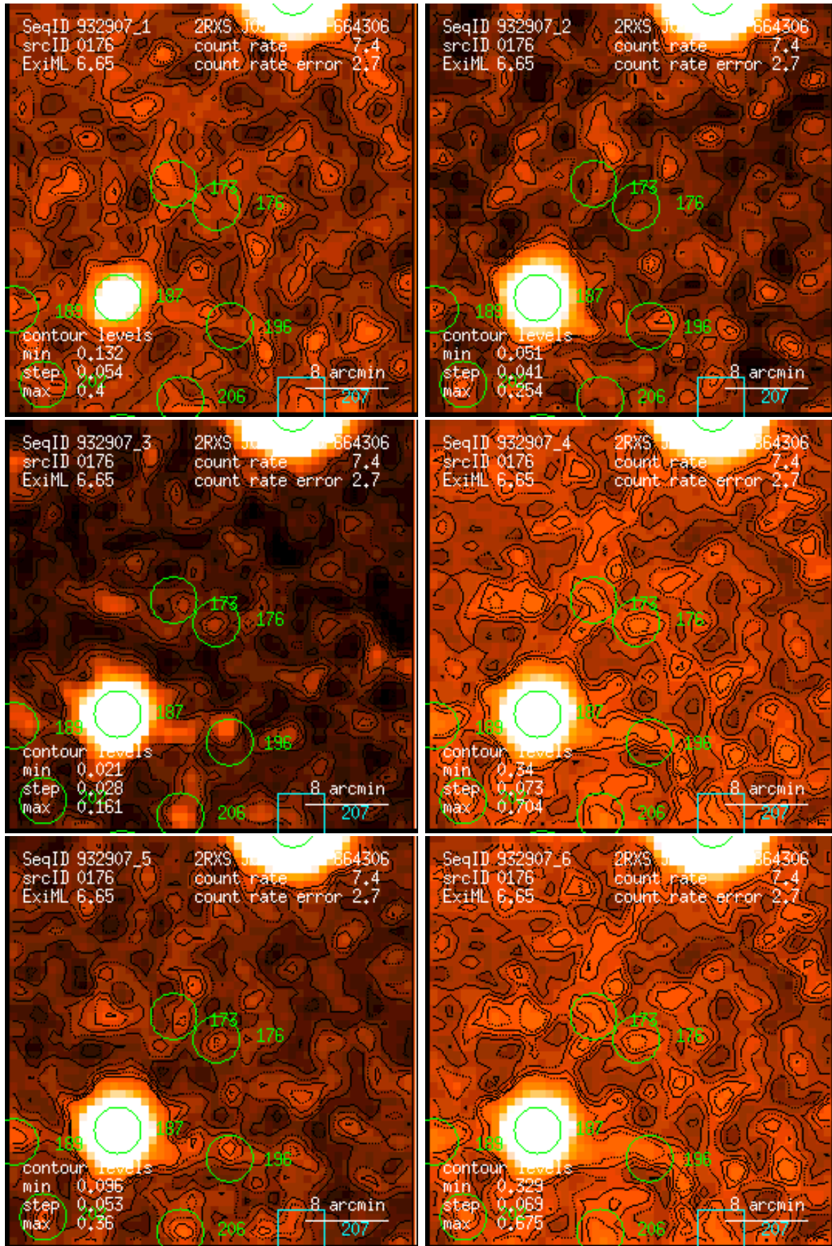
Figure 176: RASS 932907: detection 0176: band rate images, Gaussian filter: (1) PSPC channels 11 – 41, (2) 52 – 90, (3) 91 – 201, (4) 11 – 235, (5) 52 – 201, (6) 11 – 201. Broad band rates in counts/ks. Band rate contour levels in counts/ks/arcmin 2 .
