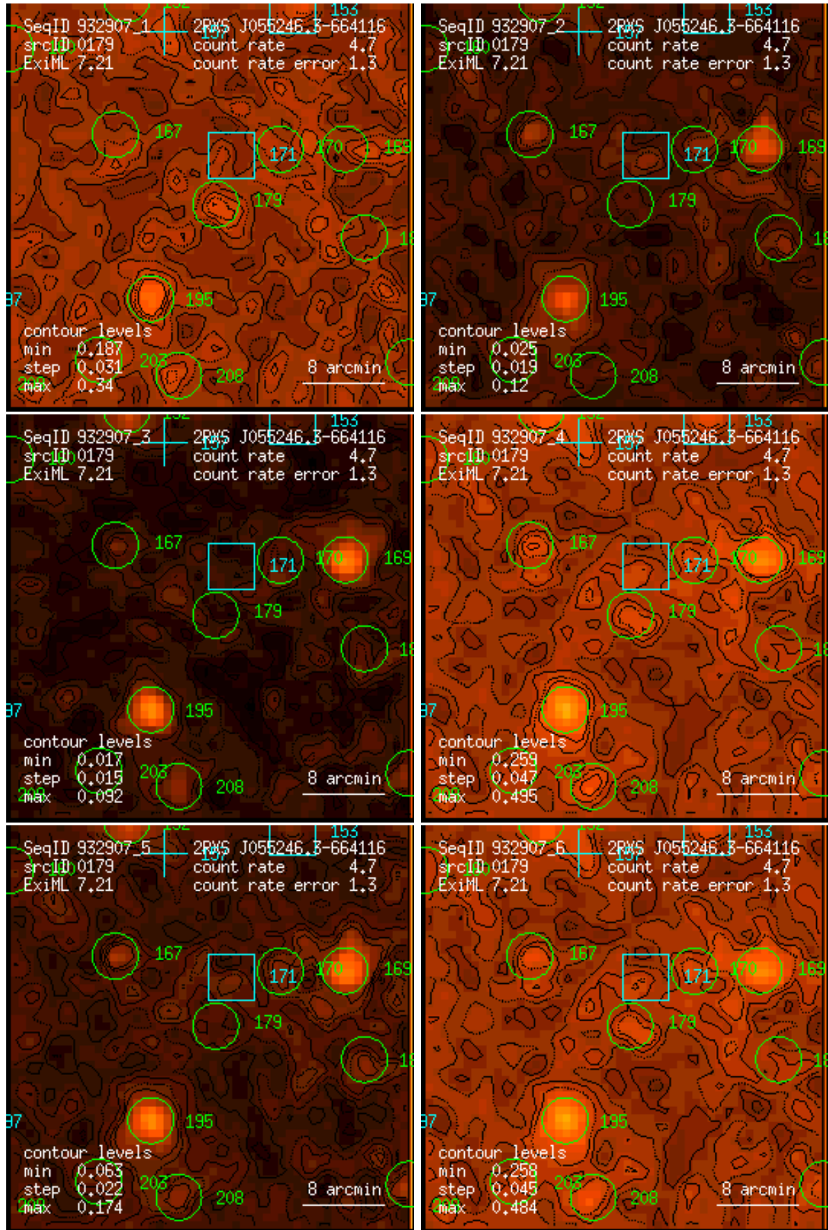
Figure 179: RASS 932907: detection 0179: band rate images, Gaussian filter: (1) PSPC channels 11 – 41, (2) 52 – 90, (3) 91 – 201, (4) 11 – 235, (5) 52 – 201, (6) 11 – 201. Broad band rates in counts/ks. Band rate contour levels in counts/ks/arcmin 2 .
