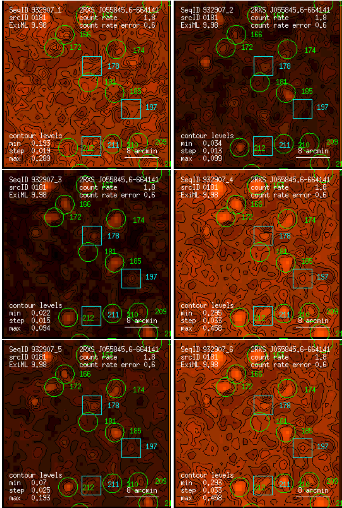
Figure 181: RASS 932907: detection 0181: band rate images, Gaussian filter: (1) PSPC channels 11 – 41, (2) 52 – 90, (3) 91 – 201, (4) 11 – 235, (5) 52 – 201, (6) 11 – 201. Broad band rates in counts/ks. Band rate contour levels in counts/ks/arcmin 2 .
