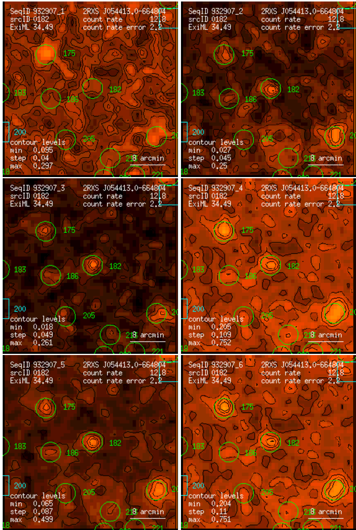
Figure 182: RASS 932907: detection 0182: band rate images, Gaussian filter: (1) PSPC channels 11 – 41, (2) 52 – 90, (3) 91 – 201, (4) 11 – 235, (5) 52 – 201, (6) 11 – 201. Broad band rates in counts/ks. Band rate contour levels in counts/ks/arcmin 2 .
