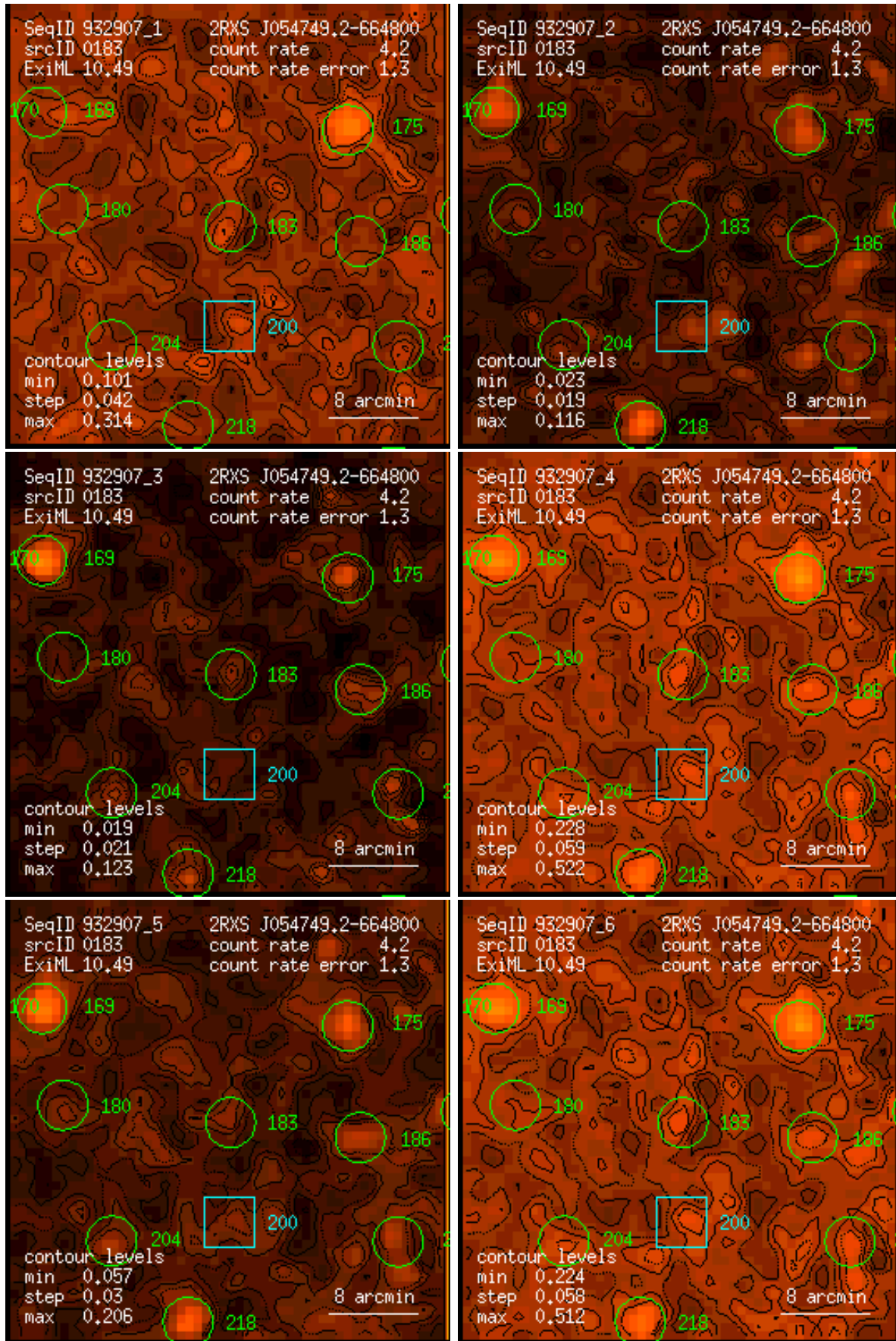
Figure 183: RASS 932907: detection 0183: band rate images, Gaussian filter: (1) PSPC channels 11 – 41, (2) 52 – 90, (3) 91 – 201, (4) 11 – 235, (5) 52 – 201, (6) 11 – 201. Broad band rates in counts/ks. Band rate contour levels in counts/ks/arcmin 2 .
