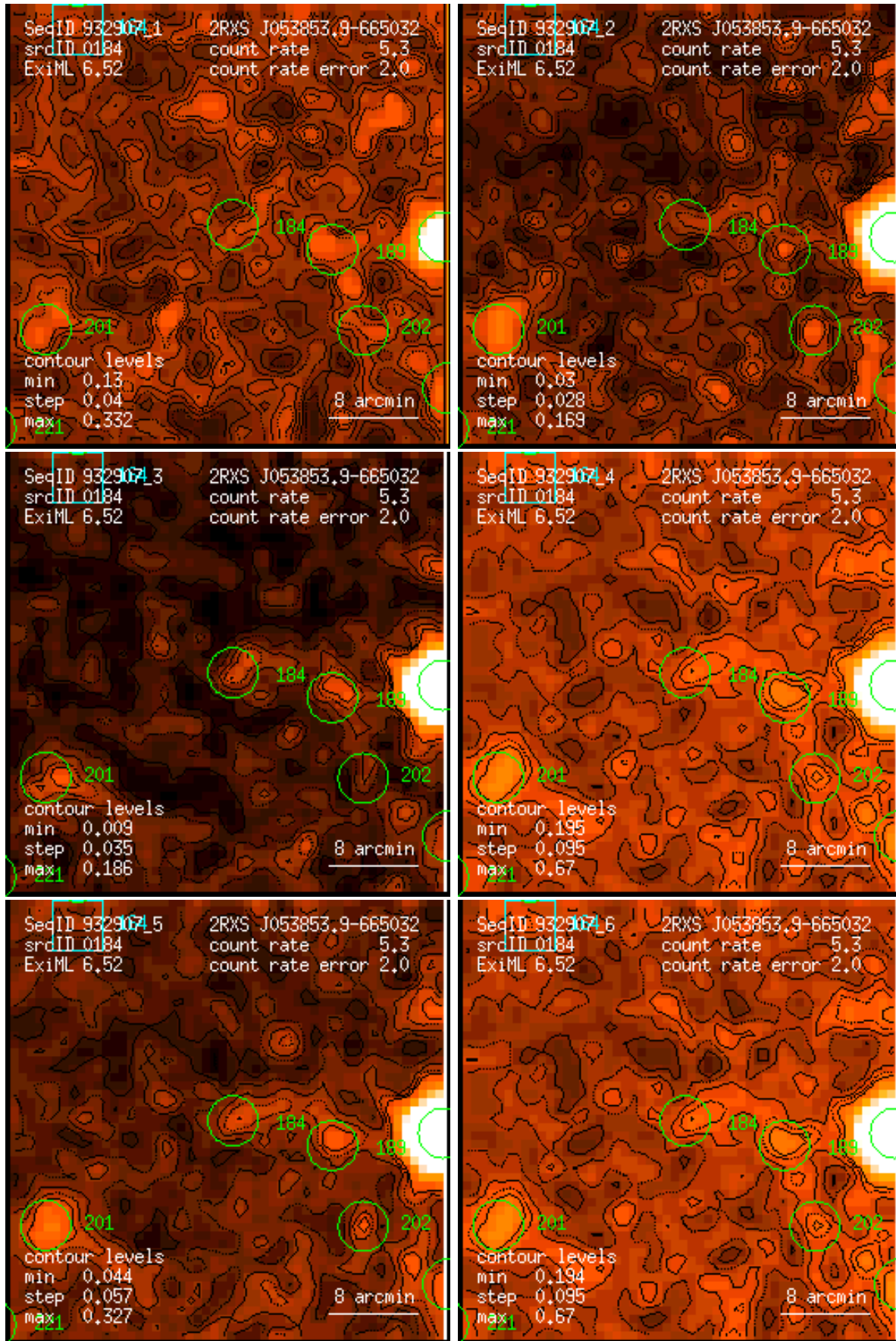
Figure 184: RASS 932907: detection 0184: band rate images, Gaussian filter: (1) PSPC channels 11 – 41, (2) 52 – 90, (3) 91 – 201, (4) 11 – 235, (5) 52 – 201, (6) 11 – 201. Broad band rates in counts/ks. Band rate contour levels in counts/ks/arcmin 2 .
