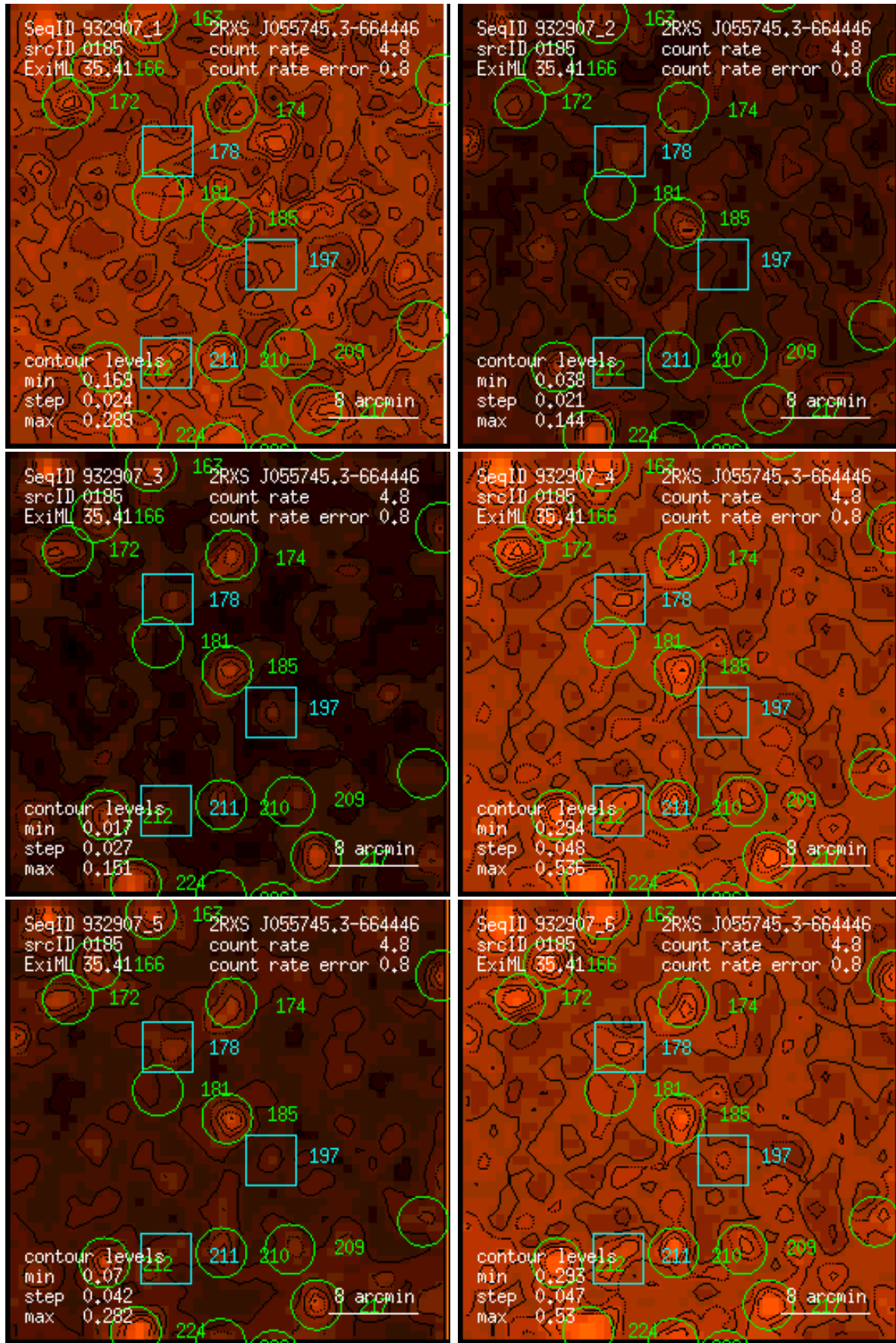
Figure 185: RASS 932907: detection 0185: band rate images, Gaussian filter: (1) PSPC channels 11 – 41, (2) 52 – 90, (3) 91 – 201, (4) 11 – 235, (5) 52 – 201, (6) 11 – 201. Broad band rates in counts/ks. Band rate contour levels in counts/ks/arcmin 2 .
