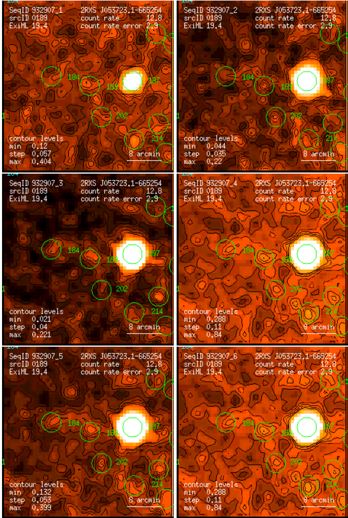
Figure 189: RASS 932907: detection 0189: band rate images, Gaussian filter: (1) PSPC channels 11 – 41, (2) 52 – 90, (3) 91 – 201, (4) 11 – 235, (5) 52 – 201, (6) 11 – 201. Broad band rates in counts/ks. Band rate contour levels in counts/ks/arcmin 2 .
