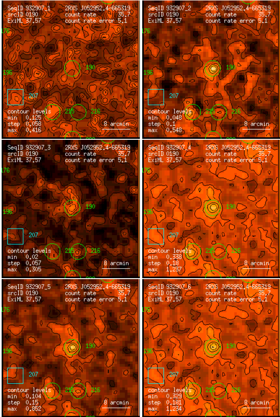
Figure 190: RASS 932907: detection 0190: band rate images, Gaussian filter: (1) PSPC channels 11 – 41, (2) 52 – 90, (3) 91 – 201, (4) 11 – 235, (5) 52 – 201, (6) 11 – 201. Broad band rates in counts/ks. Band rate contour levels in counts/ks/arcmin 2 .
