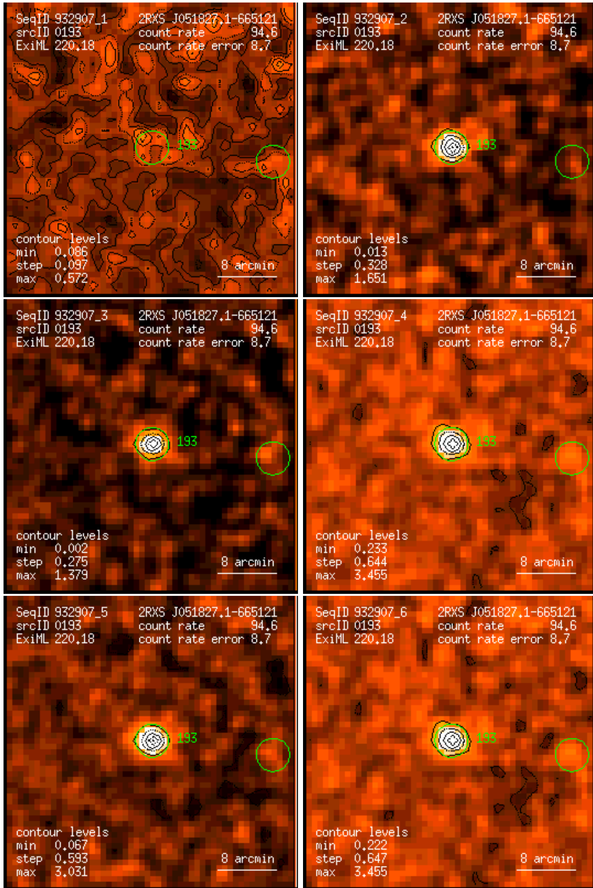
Figure 193: RASS 932907: detection 0193: band rate images, Gaussian filter: (1) PSPC channels 11 – 41, (2) 52 – 90, (3) 91 – 201, (4) 11 – 235, (5) 52 – 201, (6) 11 – 201. Broad band rates in counts/ks. Band rate contour levels in counts/ks/arcmin 2 .
