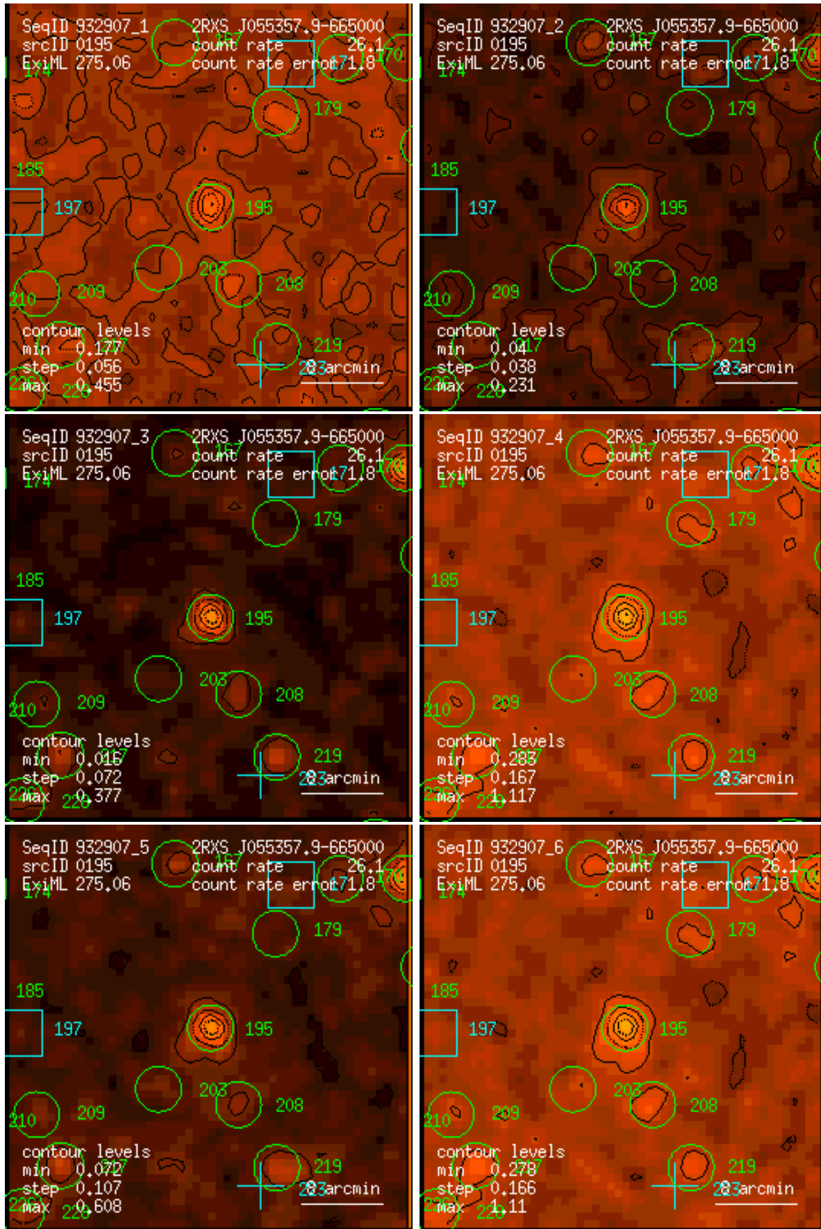
Figure 195: RASS 932907: detection 0195: band rate images, Gaussian filter: (1) PSPC channels 11 – 41, (2) 52 – 90, (3) 91 – 201, (4) 11 – 235, (5) 52 – 201, (6) 11 – 201. Broad band rates in counts/ks. Band rate contour levels in counts/ks/arcmin 2 .
