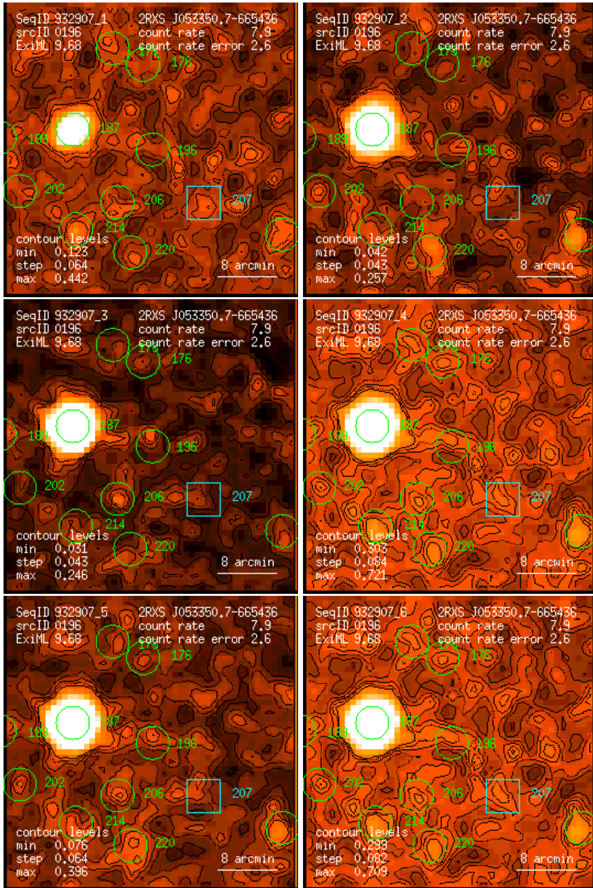
Figure 196: RASS 932907: detection 0196: band rate images, Gaussian filter: (1) PSPC channels 11 – 41, (2) 52 – 90, (3) 91 – 201, (4) 11 – 235, (5) 52 – 201, (6) 11 – 201. Broad band rates in counts/ks. Band rate contour levels in counts/ks/arcmin 2 .
